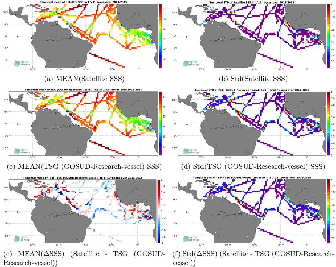
Figure 6: Temporal mean (left) and Std (right) of SSS from Aquarius SSS L3 OR v5 - Monthly - Rain mask (NASA-GSFC) (top), TSG (GOSUD-Research-vessel) (middle), and of \Delta\text{SSS} (Satellite - TSG (GOSUD-Research-vessel)). Only match-up pairs are used to generate these maps.
