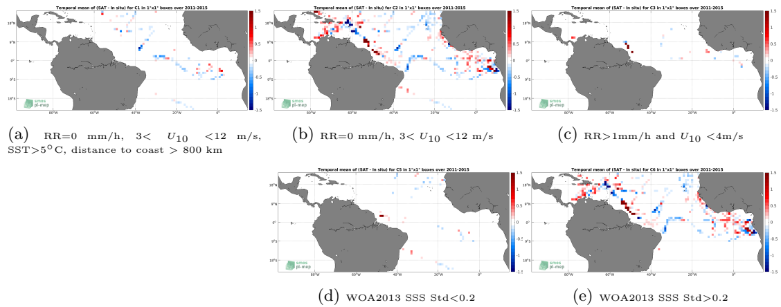
Figure 12: Temporal mean gridded over spatial boxes of size 1^\circ \times 1^\circ of \Delta SSS (Aquarius SSS L3 OR v5 - Monthly - Rain mask (NASA-GSFC) - TSG (GOSUD-Research-vessel)) for 5 different subdatasets corresponding to:RR=0 mm/h, 3 < U_{10} < 12 m/s, SST >5^\circ\text{C} , distance to coast > 800 km (a), RR=0 mm/h, 3 < U_{10} < 12 m/s (b), RR >1 mm/h and U_{10} < 4 m/s (c), WOA2013 SSS Std <0.2 (d), WOA2013 SSS Std >0.2 (e).
