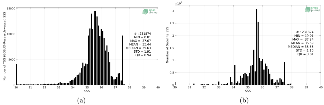
Figure 2: Histograms of SSS from TSG (GOSUD-Research-vessel) (a) and Aquarius SSS L3 OR v5 - Monthly - Rain mask (NASA-GSFC) (b) considering all match-up pairs per bins of 0.1 over the Tropical Atlantic Ocean Pi-MEP region and for the full satellite product period.
