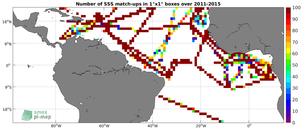
Figure 4: Number of SSS match-ups between TSG (GOSUD-Research-vessel) SSS and the Aquarius SSS L3 OR v5 - Monthly - Rain mask (NASA-GSFC) SSS product for the Tropical Atlantic Ocean Pi-MEP region over 1^\circ \times 1^\circ boxes and for the full satellite product period.
