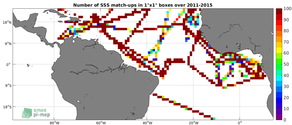
Figure 4: Number of SSS match-ups between TSG-GOSUD-Research-vessel SSS and the Aquarius-L3-OR-V5-MONTHLY-RAIN-MASK-1DEG SSS product for the Tropical Atlantic Ocean Pi-MEP region over 1°x1° boxes and for the full satellite product period.
