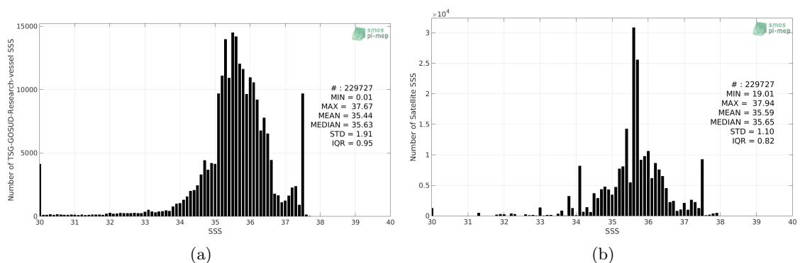
Figure 2: Histograms of SSS from TSG-GOSUD-Research-vessel (a) and Aquarius-L3-OR-V5-MONTHLY-RAIN-MASK-1DEG (b) considering all match-up pairs per bins of 0.1 over the Tropical Atlantic Ocean Pi-MEP region and for the full satellite product period.
