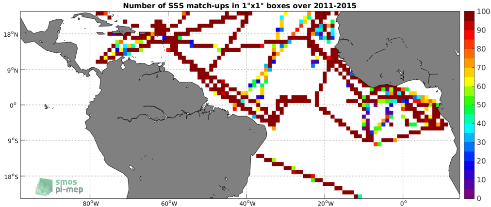
Figure 4: Number of SSS match-ups between TSG-GOSUD-Research-vessel SSS and the Aquarius-L3-OR-V5-MONTHLY-RAIN-MASK-1DEG SSS product for the Tropical Atlantic Ocean Pi-MEP region over 1^\circ \times 1^\circ boxes and for the full satellite product period.
