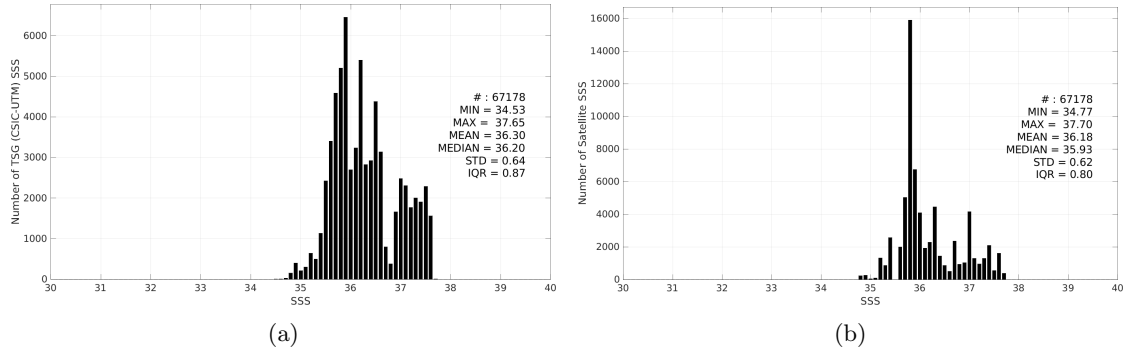
Figure 3: Histograms of SSS from TSG (CSIC-UTM) (a) and Aquarius SSS L3 OR v5 - Monthly - Rain mask (NASA-GSFC) (b) considering all match-up pairs per bins of 0.1 over the Tropical Atlantic Ocean Pi-MEP region and for the full satellite product period.
