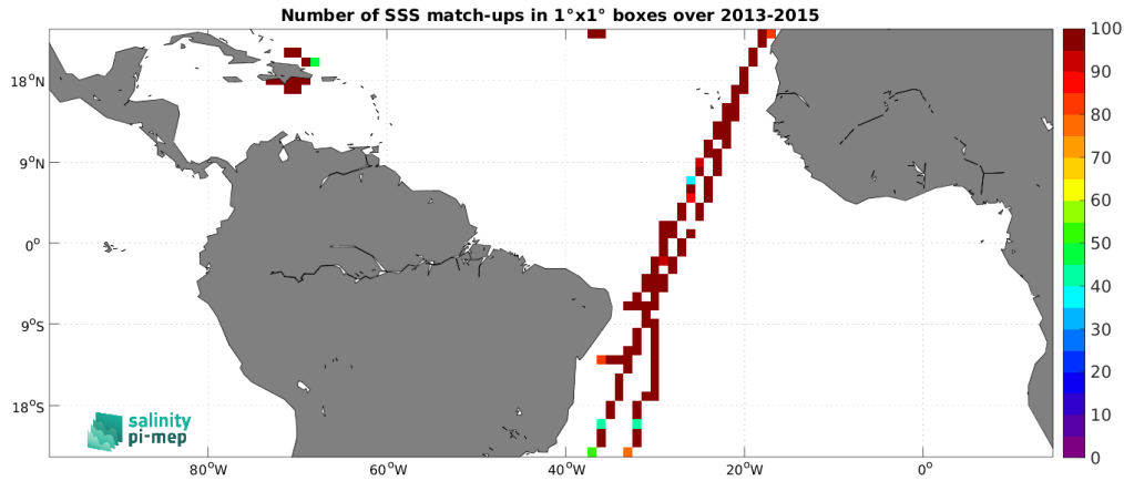
Figure 5: Number of SSS match-ups between TSG (CSIC-UTM) SSS and the Aquarius SSS L3 OR v5 - Monthly - Rain mask (NASA-GSFC) SSS product for the Tropical Atlantic Ocean Pi-MEP region over 1^\circ \times 1^\circ boxes and for the full satellite product period.
