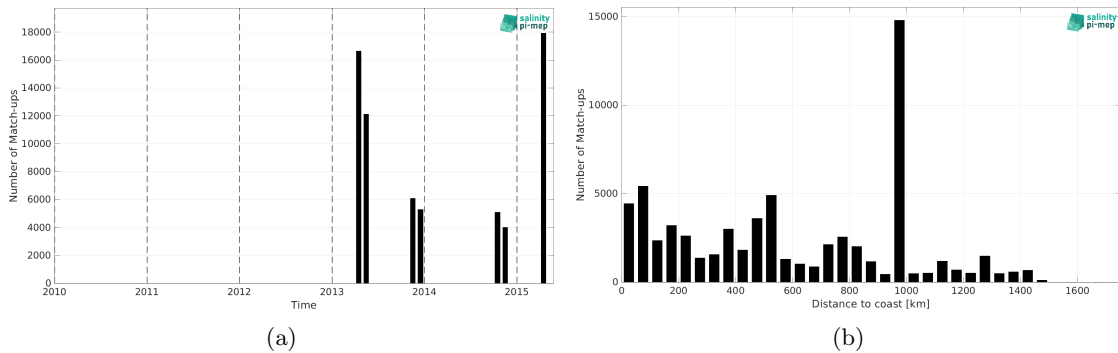
Figure 2: Number of match-ups between TSG (CSIC-UTM) and Aquarius SSS L3 OR v5 - Monthly - Rain mask (NASA-GSFC) SSS as a function of time (a) and as function of the distance to coast (b) over the Tropical Atlantic Ocean Pi-MEP region and for the full satellite product period.
