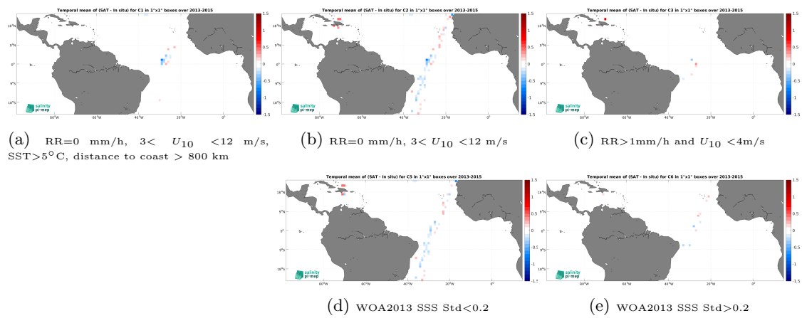
Figure 14: Temporal mean gridded over spatial boxes of size 1^\circ \times 1^\circ of \Delta SSS (Aquarius SSS L3 OR v5 - Monthly - Rain mask (NASA-GSFC) - TSG (CSIC-UTM)) for 5 different subdatasets corresponding to:RR=0 mm/h, 3 < U_{10} < 12 m/s, SST >5^\circ\text{C} , distance to coast > 800 km (a), RR=0 mm/h, 3 < U_{10} < 12 m/s (b), RR >1 mm/h and U_{10} < 4 m/s (c), WOA2013 SSS Std <0.2 (d), WOA2013 SSS Std >0.2 (e).
