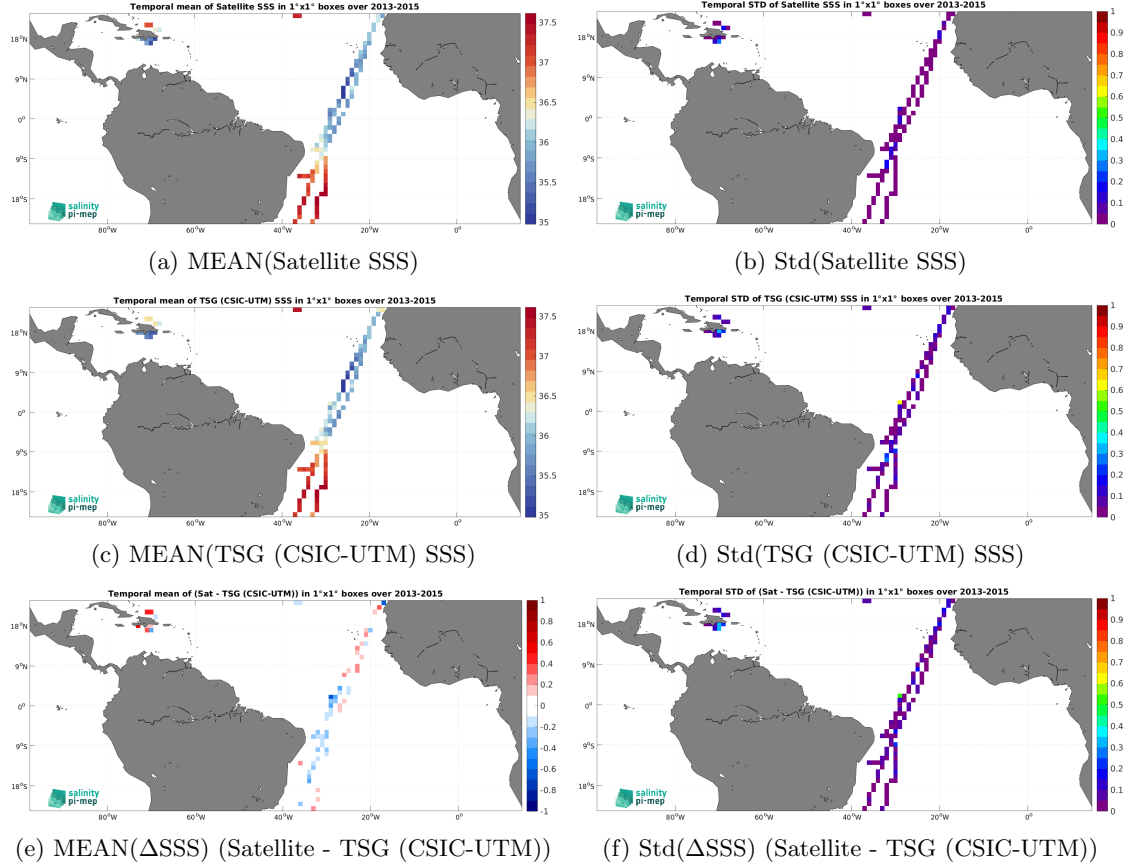
Figure 7: Temporal mean (left) and Std (right) of SSS from Aquarius SSS L3 OR v5 - Monthly - Rain mask (NASA-GSFC) (top), TSG (CSIC-UTM) (middle), and of \Delta\text{SSS} (Satellite - TSG (CSIC-UTM)). Only match-up pairs are used to generate these maps.
