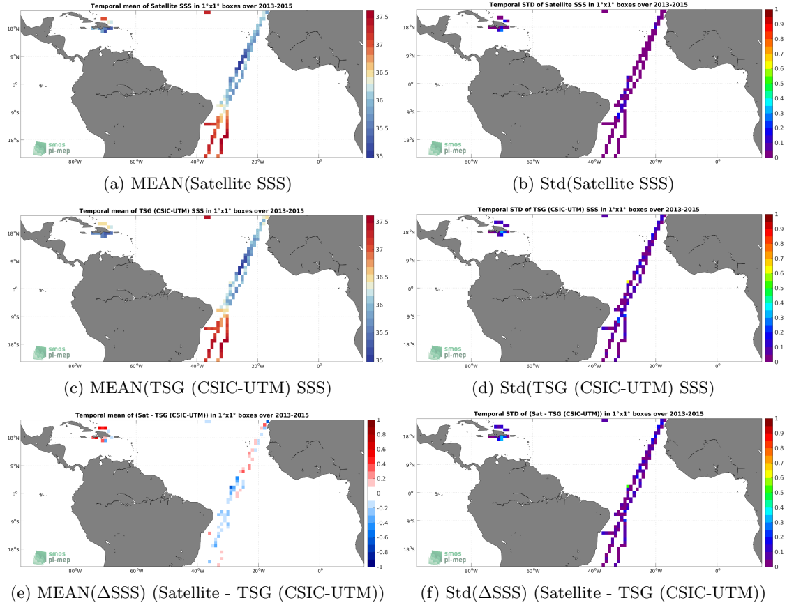
Figure 6: Temporal mean (left) and Std (right) of SSS from Aquarius SSS L3 OR v5 - Monthly - Rain mask (NASA-GSFC) (top), TSG (CSIC-UTM) (middle), and of \Delta\text{SSS} (Satellite - TSG (CSIC-UTM)). Only match-up pairs are used to generate these maps.
