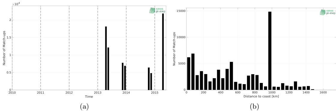
Figure 1: Number of match-ups between TSG (CSIC-UTM) and Aquarius SSS L3 OR v5 - Monthly - Rain mask (NASA-GSFC) SSS as a function of time (a) and as function of the distance to coast (b) over the Tropical Atlantic Ocean Pi-MEP region and for the full satellite product period.
