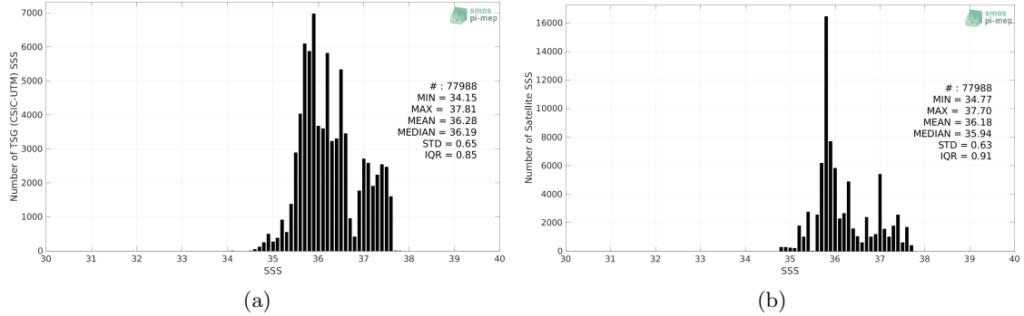
Figure 2: Histograms of SSS from TSG (CSIC-UTM) (a) and Aquarius SSS L3 OR v5 - Monthly - Rain mask (NASA-GSFC) (b) considering all match-up pairs per bins of 0.1 over the Tropical Atlantic Ocean Pi-MEP region and for the full satellite product period.
