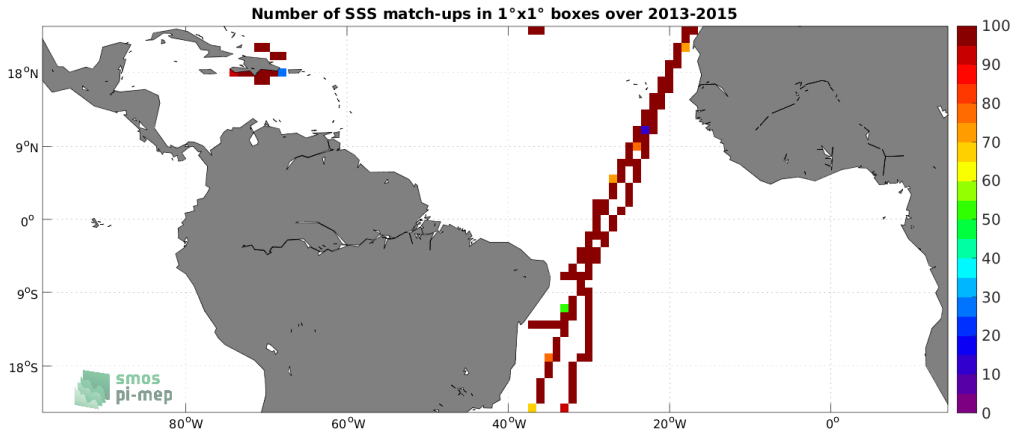
Figure 4: Number of SSS match-ups between TSG (CSIC-UTM) SSS and the Aquarius SSS L3 OR v5 - Monthly - Rain mask (NASA-GSFC) SSS product for the Tropical Atlantic Ocean Pi-MEP region over 1^\circ \times 1^\circ boxes and for the full satellite product period.
