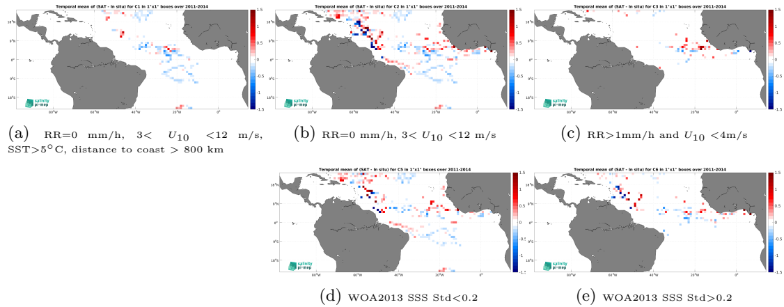
Figure 11: Temporal mean gridded over spatial boxes of size 1^\circ \times 1^\circ of \Delta SSS (Aquarius SSS L3 OR v5 - Monthly - Rain mask (NASA-GSFC) - Surface drifters) for 5 different subdatasets corresponding to:RR=0 mm/h, 3 < U_{10} < 12 m/s, SST >5^\circ\text{C} , distance to coast > 800 km (a), RR=0 mm/h, 3 < U_{10} < 12 m/s (b), RR >1 mm/h and U_{10} < 4 m/s (c), WOA2013 SSS Std <0.2 (d), WOA2013 SSS Std >0.2 (e).
