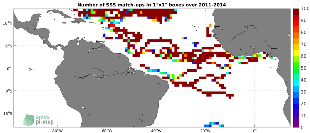
Figure 3: Number of SSS match-ups between Surface drifters SSS and the Aquarius SSS L3 OR v5 - Monthly - Rain mask (NASA-GSFC) SSS product for the Tropical Atlantic Ocean Pi-MEP region over 1^\circ \times 1^\circ boxes and for the full satellite product period.
