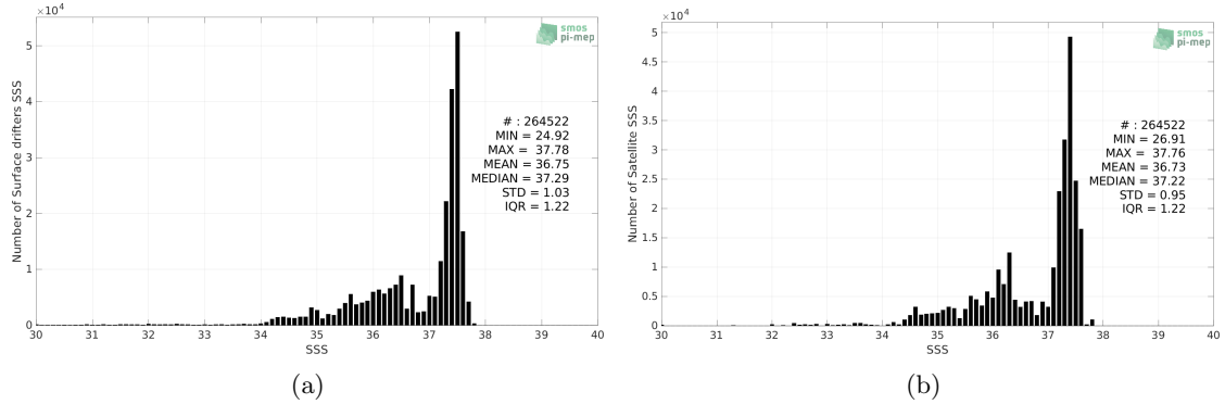
Figure 2: Histograms of SSS from Surface drifters (a) and Aquarius SSS L3 OR v5 - Monthly - Rain mask (NASA-GSFC) (b) considering all match-up pairs per bins of 0.1 over the Tropical Atlantic Ocean Pi-MEP region and for the full satellite product period.
