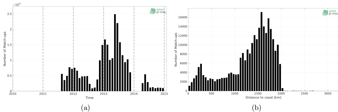
Figure 1: Number of match-ups between Surface drifters and Aquarius SSS L3 OR v5 - Monthly - Rain mask (NASA-GSFC) SSS as a function of time (a) and as function of the distance to coast (b) over the Tropical Atlantic Ocean Pi-MEP region and for the full satellite product period.
