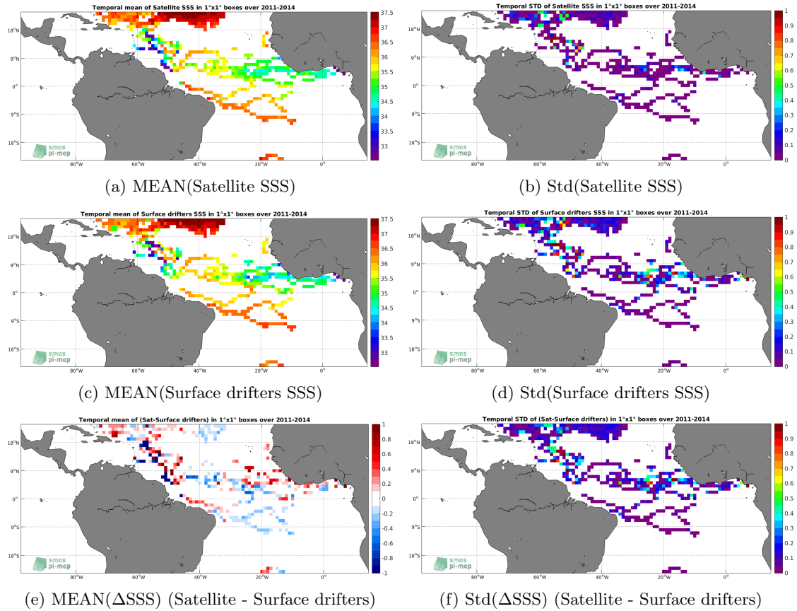
Figure 5: Temporal mean (left) and Std (right) of SSS from Aquarius-L3-OR-V5-MONTHLY-RAIN-MASK-1DEG (top), Surface drifters (middle), and of \Delta SSS (Satellite - Surface drifters). Only match-up pairs are used to generate these maps.
