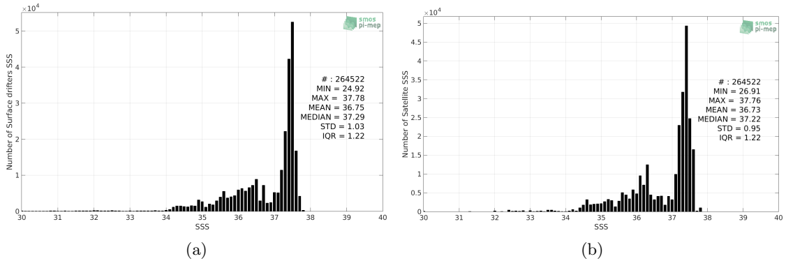
Figure 2: Histograms of SSS from Surface drifters (a) and Aquarius-L3-OR-V5-MONTHLY-RAIN-MASK-1DEG (b) considering all match-up pairs per bins of 0.1 over the Tropical Atlantic Ocean Pi-MEP region and for the full satellite product period.
