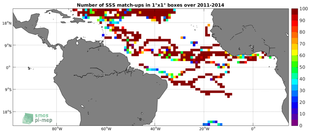
Figure 3: Number of SSS match-ups between Surface drifters SSS and the Aquarius-L3-OR-V5-MONTHLY-RAIN-MASK-1DEG SSS product for the Tropical Atlantic Ocean Pi-MEP region over 1°x1° boxes and for the full satellite product period.
