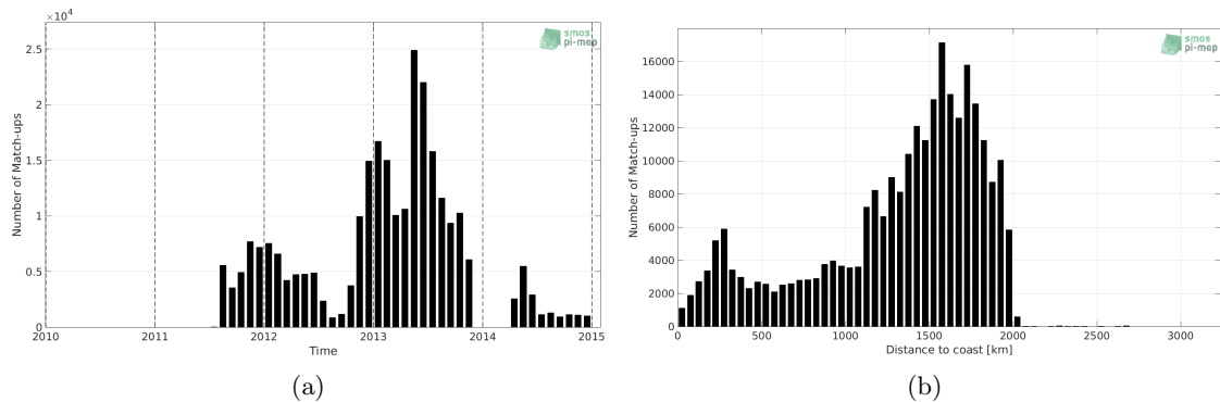
Figure 1: Number of match-ups between Surface drifters and Aquarius-L3-OR-V5-MONTHLY-RAIN-MASK-1DEG SSS as a function of time (a) and as function of the distance to coast (b) over the Tropical Atlantic Ocean Pi-MEP region and for the full satellite product period.
