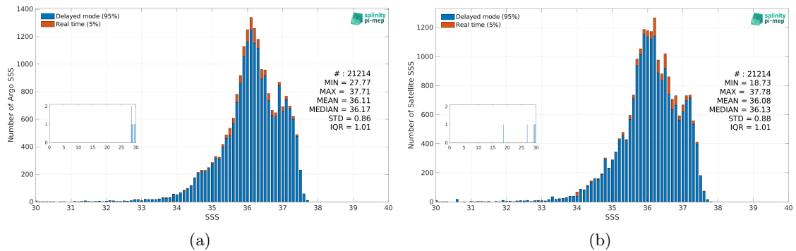
Figure 3: Histograms of SSS from Argo (a) and Aquarius SSS L3 OR v5 - Monthly - Rain mask (NASA-GSFC) (b) considering all match-up pairs per bins of 0.1 over the Tropical Atlantic Ocean Pi-MEP region and for the full satellite product period.
