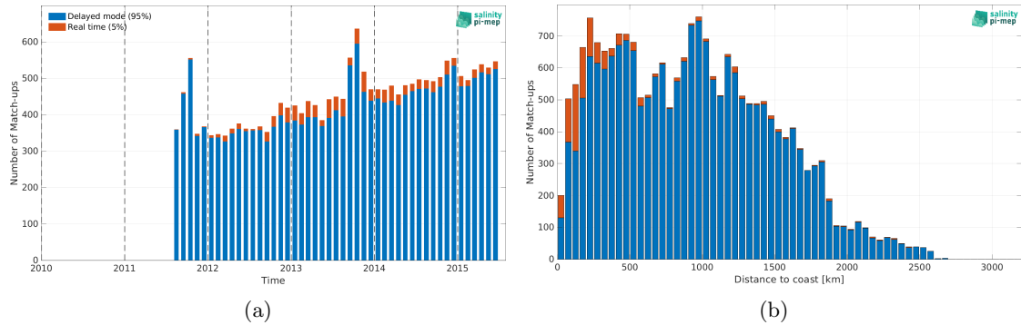
Figure 2: Number of match-ups between Argo and Aquarius SSS L3 OR v5 - Monthly - Rain mask (NASA-GSFC) SSS as a function of time (a) and as function of the distance to coast (b) over the Tropical Atlantic Ocean Pi-MEP region and for the full satellite product period.
