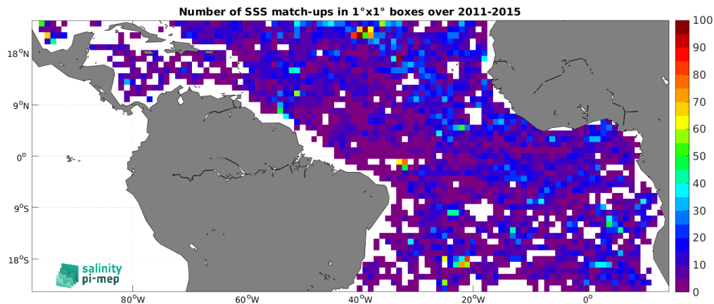
Figure 5: Number of SSS match-ups between Argo SSS and the Aquarius SSS L3 OR v5 - Monthly - Rain mask (NASA-GSFC) SSS product for the Tropical Atlantic Ocean Pi-MEP region over 1^\circ \times 1^\circ boxes and for the full satellite product period.
