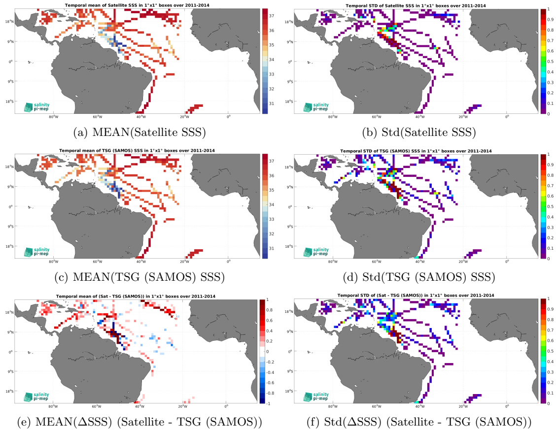
Figure 7: Temporal mean (left) and Std (right) of SSS from Aquarius SSS L3 CAP v5 - 7-Day running (JPL) (top), TSG (SAMOS) (middle), and of \Delta SSS (Satellite - TSG (SAMOS)). Only match-up pairs are used to generate these maps.
