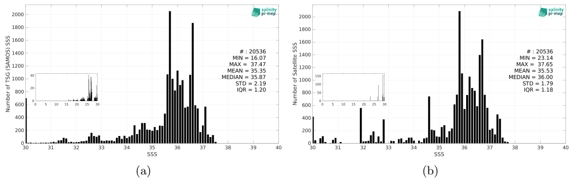
Figure 3: Histograms of SSS from TSG (SAMOS) (a) and Aquarius SSS L3 CAP v5 - 7-Day running (JPL) (b) considering all match-up pairs per bins of 0.1 over the Tropical Atlantic Ocean Pi-MEP region and for the full satellite product period.
