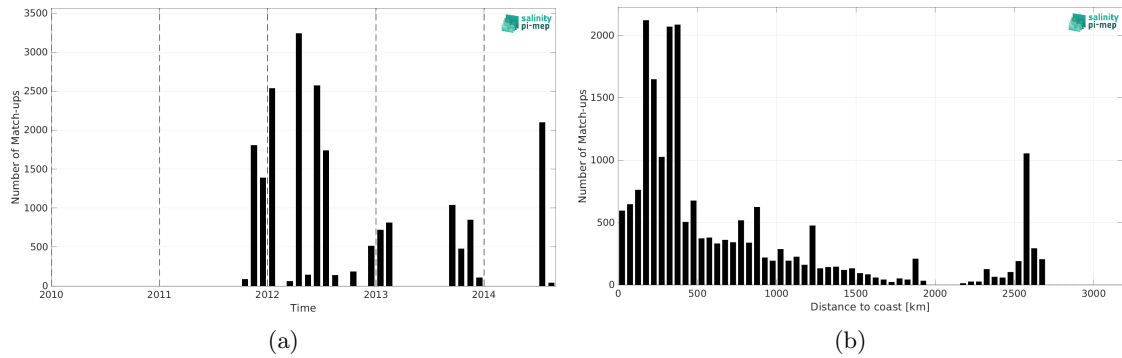
Figure 2: Number of match-ups between TSG (SAMOS) and Aquarius SSS L3 CAP v5 - 7-Day running (JPL) SSS as a function of time (a) and as function of the distance to coast (b) over the Tropical Atlantic Ocean Pi-MEP region and for the full satellite product period.
