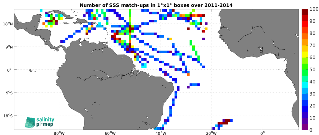
Figure 5: Number of SSS match-ups between TSG (SAMOS) SSS and the Aquarius SSS L3 CAP v5 - 7-Day running (JPL) SSS product for the Tropical Atlantic Ocean Pi-MEP region over 1^\circ \times 1^\circ boxes and for the full satellite product period.
