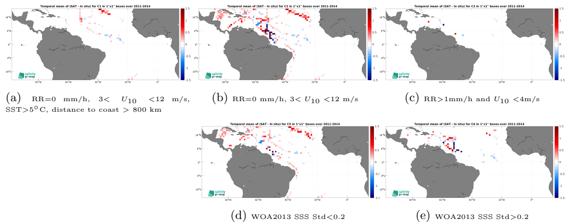
Figure 14: Temporal mean gridded over spatial boxes of size 1^\circ \times 1^\circ of \Delta SSS (Aquarius SSS L3 CAP v5 - 7-Day running (JPL) - TSG (SAMOS)) for 5 different subdatasets corresponding to:RR=0 mm/h, 3 < U_{10} < 12 m/s, SST >5^\circ\text{C} , distance to coast > 800 km (a), RR=0 mm/h, 3 < U_{10} < 12 m/s (b), RR >1 mm/h and U_{10} < 4 m/s (c), WOA2013 SSS Std <0.2 (d), WOA2013 SSS Std >0.2 (e).
