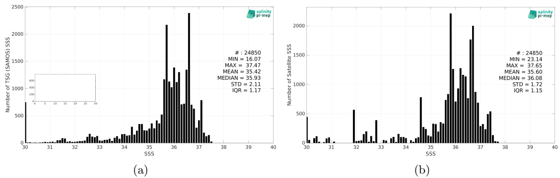
Figure 2: Histograms of SSS from TSG (SAMOS) (a) and Aquarius SSS L3 CAP v5 - 7-Day running (JPL) (b) considering all match-up pairs per bins of 0.1 over the Tropical Atlantic Ocean Pi-MEP region and for the full satellite product period.
