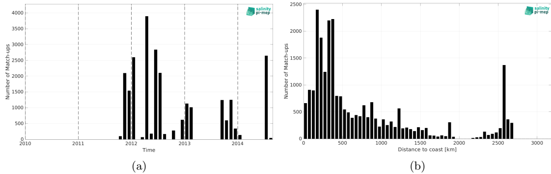
Figure 1: Number of match-ups between TSG (SAMOS) and Aquarius SSS L3 CAP v5 - 7-Day running (JPL) SSS as a function of time (a) and as function of the distance to coast (b) over the Tropical Atlantic Ocean Pi-MEP region and for the full satellite product period.
