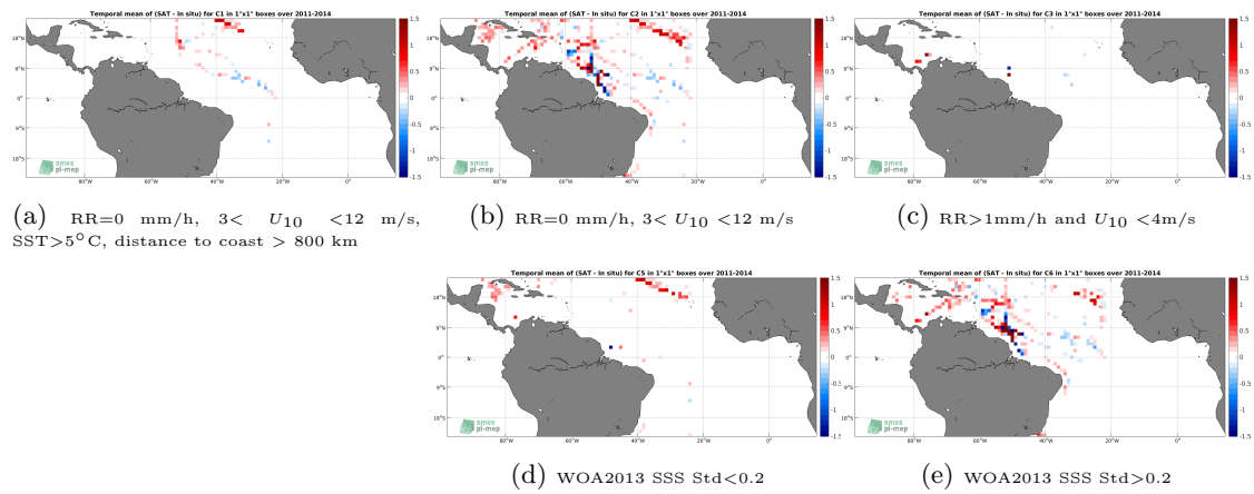
Figure 12: Temporal mean gridded over spatial boxes of size 1^\circ \times 1^\circ of \Delta SSS (Aquarius-L3-JPL-V5-7DAY-RUNNING - TSG-SAMOS) for 5 different subdatasets corresponding to: RR=0 mm/h, 3 < U_{10} < 12 m/s, SST > 5^\circ\text{C} , distance to coast > 800 km (a), RR=0 mm/h, 3 < U_{10} < 12 m/s (b), RR > 1 mm/h and U_{10} < 4 m/s (c), WOA2013 SSS Std < 0.2 (d), WOA2013 SSS Std > 0.2 (e).
