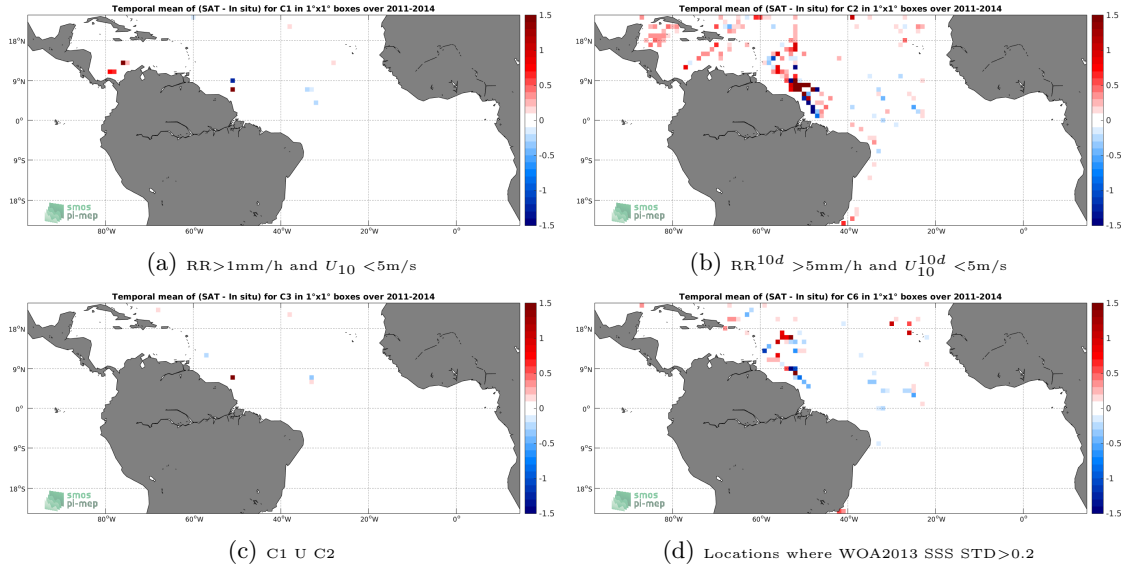
Figure 12: Temporal mean gridded over spatial boxes of size 1^\circ \times 1^\circ of \Delta SSS (Aquarius-L3-JPL-V5-7DAY-RUNNING - TSG-SAMOS) for 4 different subdatasets corresponding to: RR > 1mm/h and U_{10} < 5\text{m/s} (a), RR^{10d} > 5\text{mm/h} and U_{10}^{10d} < 5\text{m/s} (b), C1 U C2 (c), Locations where WOA2013 SSS STD > 0.2 (d).
