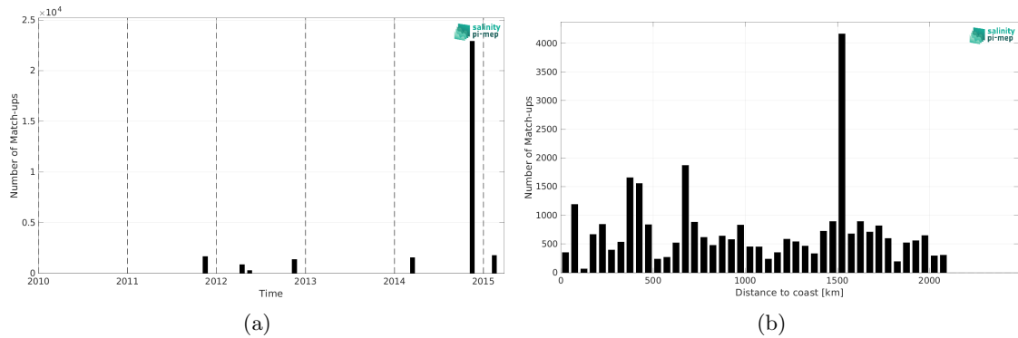
Figure 2: Number of match-ups between TSG (Polarstern) and Aquarius SSS L3 CAP v5 - 7-Day running (JPL) SSS as a function of time (a) and as function of the distance to coast (b) over the Tropical Atlantic Ocean Pi-MEP region and for the full satellite product period.
