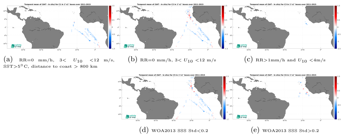
Figure 14: Temporal mean gridded over spatial boxes of size 1^\circ \times 1^\circ of \Delta SSS (Aquarius SSS L3 CAP v5 - 7-Day running (JPL) - TSG (Polarstern)) for 5 different subdatasets corresponding to:RR=0 mm/h, 3 < U_{10} < 12 m/s, SST >5^\circ\text{C} , distance to coast > 800 km (a), RR=0 mm/h, 3 < U_{10} < 12 m/s (b), RR >1 mm/h and U_{10} < 4 m/s (c), WOA2013 SSS Std <0.2 (d), WOA2013 SSS Std >0.2 (e).
