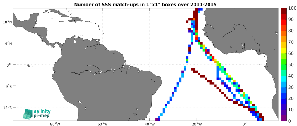
Figure 5: Number of SSS match-ups between TSG (Polarstern) SSS and the Aquarius SSS L3 CAP v5 - 7-Day running (JPL) SSS product for the Tropical Atlantic Ocean Pi-MEP region over 1^\circ \times 1^\circ boxes and for the full satellite product period.
