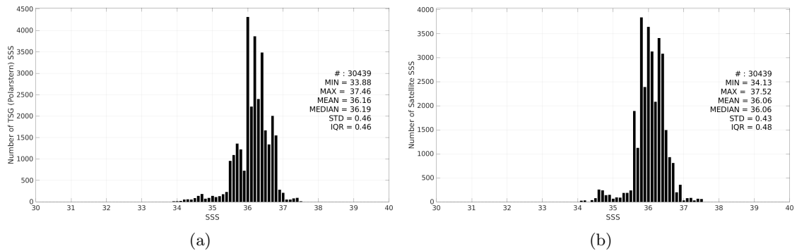
Figure 3: Histograms of SSS from TSG (Polarstern) (a) and Aquarius SSS L3 CAP v5 - 7-Day running (JPL) (b) considering all match-up pairs per bins of 0.1 over the Tropical Atlantic Ocean Pi-MEP region and for the full satellite product period.
