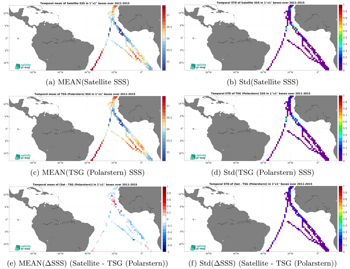
Figure 7: Temporal mean (left) and Std (right) of SSS from Aquarius SSS L3 CAP v5 - 7-Day running (JPL) (top), TSG (Polarstern) (middle), and of \Delta SSS (Satellite - TSG (Polarstern)). Only match-up pairs are used to generate these maps.
