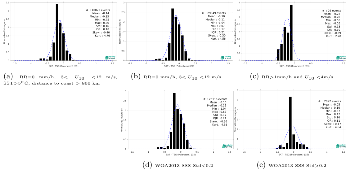
Figure 15: Normalized histogram of \Delta\text{SSS} (Aquarius SSS L3 CAP v5 - 7-Day running (JPL) - TSG (Polarstern)) for 5 different subdatasets corresponding to: RR=0 mm/h, 3 < U_{10} < 12 m/s, SST>5°C, distance to coast > 800 km (a), RR=0 mm/h, 3 < U_{10} < 12 m/s (b), RR>1mm/h and U_{10} < 4 m/s (c), WOA2013 SSS Std<0.2 (d), WOA2013 SSS Std>0.2 (e).
