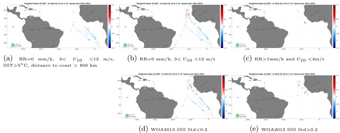
Figure 12: Temporal mean gridded over spatial boxes of size 1^\circ \times 1^\circ of \Delta\text{SSS} (Aquarius SSS L3 CAP v5 - 7-Day running (JPL) - TSG (Polarstern)) for 5 different subdatasets corresponding to:RR=0 mm/h, 3 < U_{10} < 12 m/s, SST >5^\circ\text{C} , distance to coast > 800 km (a), RR=0 mm/h, 3 < U_{10} < 12 m/s (b), RR >1 mm/h and U_{10} < 4 m/s (c), WOA2013 SSS Std <0.2 (d), WOA2013 SSS Std >0.2 (e).
