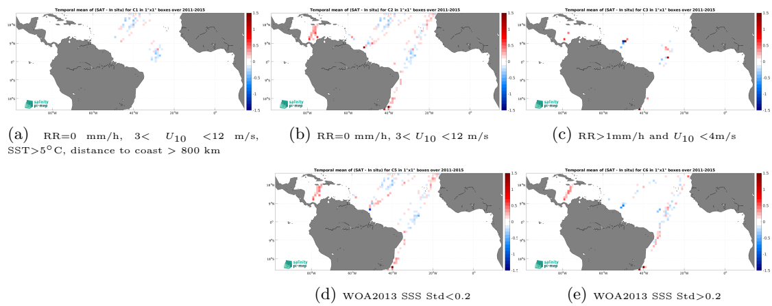
Figure 14: Temporal mean gridded over spatial boxes of size 1^\circ \times 1^\circ of \Delta SSS (Aquarius SSS L3 CAP v5 - 7-Day running (JPL) - TSG (LEGOS-DM)) for 5 different subdatasets corresponding to:RR=0 mm/h, 3 < U_{10} < 12 m/s, SST >5^\circ\text{C} , distance to coast > 800 km (a), RR=0 mm/h, 3 < U_{10} < 12 m/s (b), RR >1 mm/h and U_{10} < 4 m/s (c), WOA2013 SSS Std <0.2 (d), WOA2013 SSS Std >0.2 (e).
