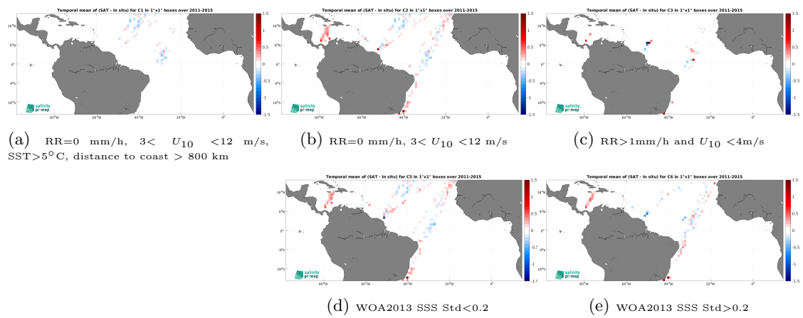
Figure 14: Temporal mean gridded over spatial boxes of size 1^\circ \times 1^\circ of \Delta\text{SSS} (Aquarius SSS L3 CAP v5 - 7-Day running (JPL) - TSG (LEGOS-DM)) for 5 different subdatasets corresponding to:RR=0 mm/h, 3 < U_{10} < 12 m/s, SST>5°C, distance to coast > 800 km (a), RR=0 mm/h, 3 < U_{10} < 12 m/s (b), RR>1mm/h and U_{10} < 4 m/s (c), WOA2013 SSS Std<0.2 (d), WOA2013 SSS Std>0.2 (e).
