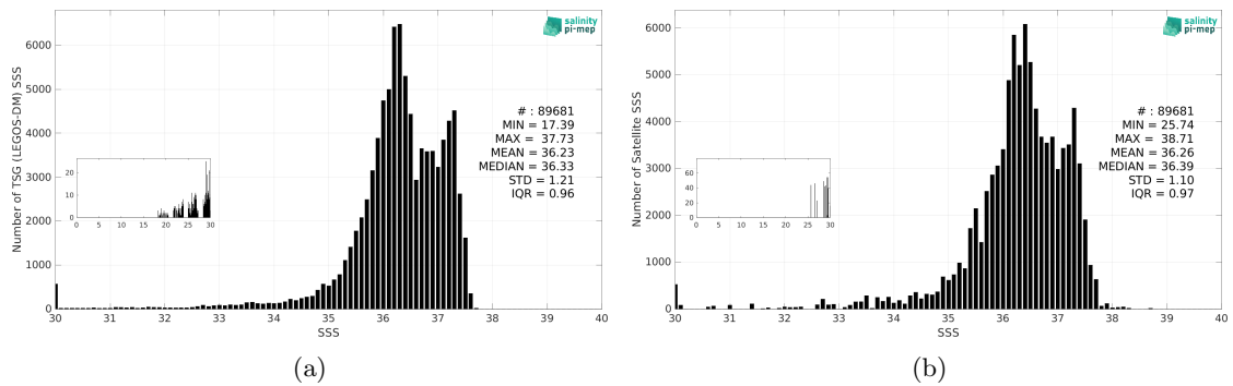
Figure 3: Histograms of SSS from TSG (LEGOS-DM) (a) and Aquarius SSS L3 CAP v5 - 7-Day running (JPL) (b) considering all match-up pairs per bins of 0.1 over the Tropical Atlantic Ocean Pi-MEP region and for the full satellite product period.
