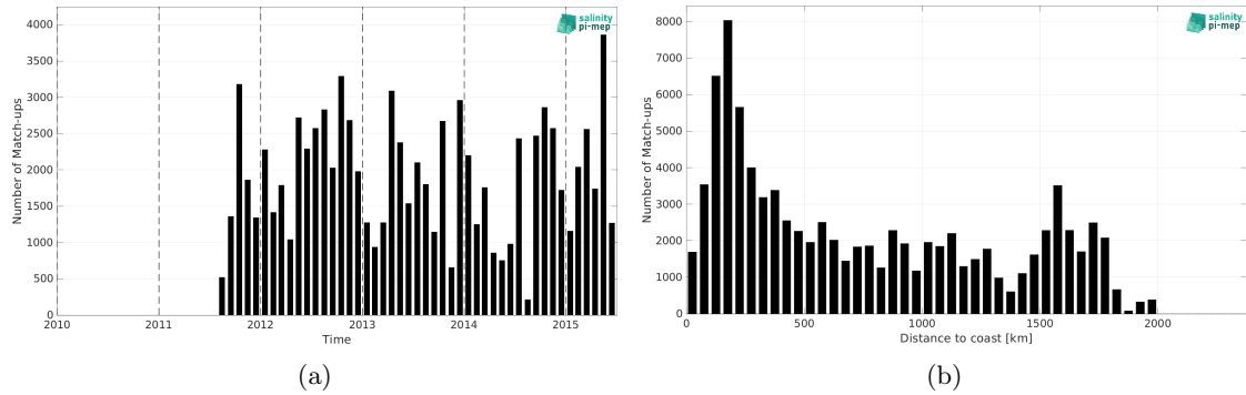
Figure 2: Number of match-ups between TSG (LEGOS-DM) and Aquarius SSS L3 CAP v5 - 7-Day running (JPL) SSS as a function of time (a) and as function of the distance to coast (b) over the Tropical Atlantic Ocean Pi-MEP region and for the full satellite product period.
