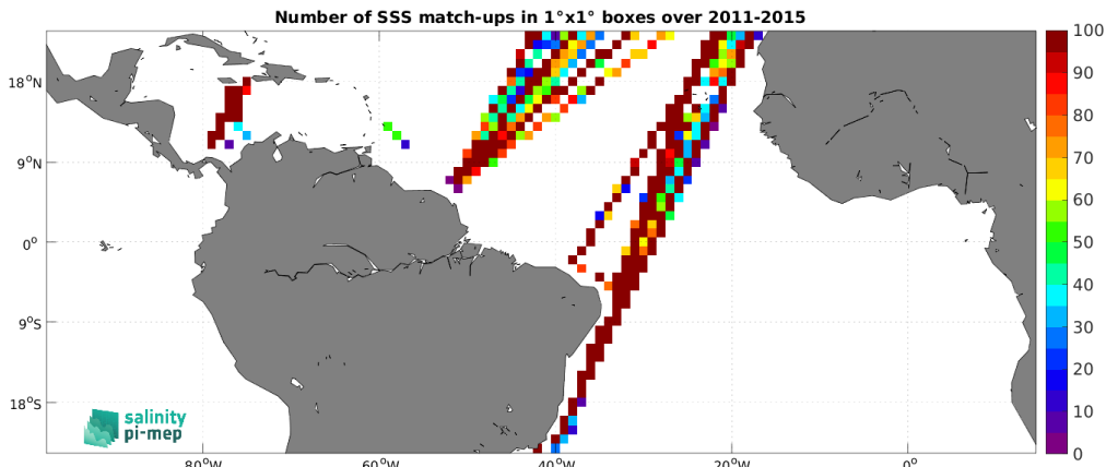
Figure 5: Number of SSS match-ups between TSG (LEGOS-DM) SSS and the Aquarius SSS L3 CAP v5 - 7-Day running (JPL) SSS product for the Tropical Atlantic Ocean Pi-MEP region over 1^\circ \times 1^\circ boxes and for the full satellite product period.
