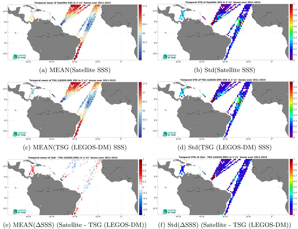
Figure 7: Temporal mean (left) and Std (right) of SSS from Aquarius SSS L3 CAP v5 - 7-Day running (JPL) (top), TSG (LEGOS-DM) (middle), and of \Delta SSS (Satellite - TSG (LEGOS-DM)). Only match-up pairs are used to generate these maps.
