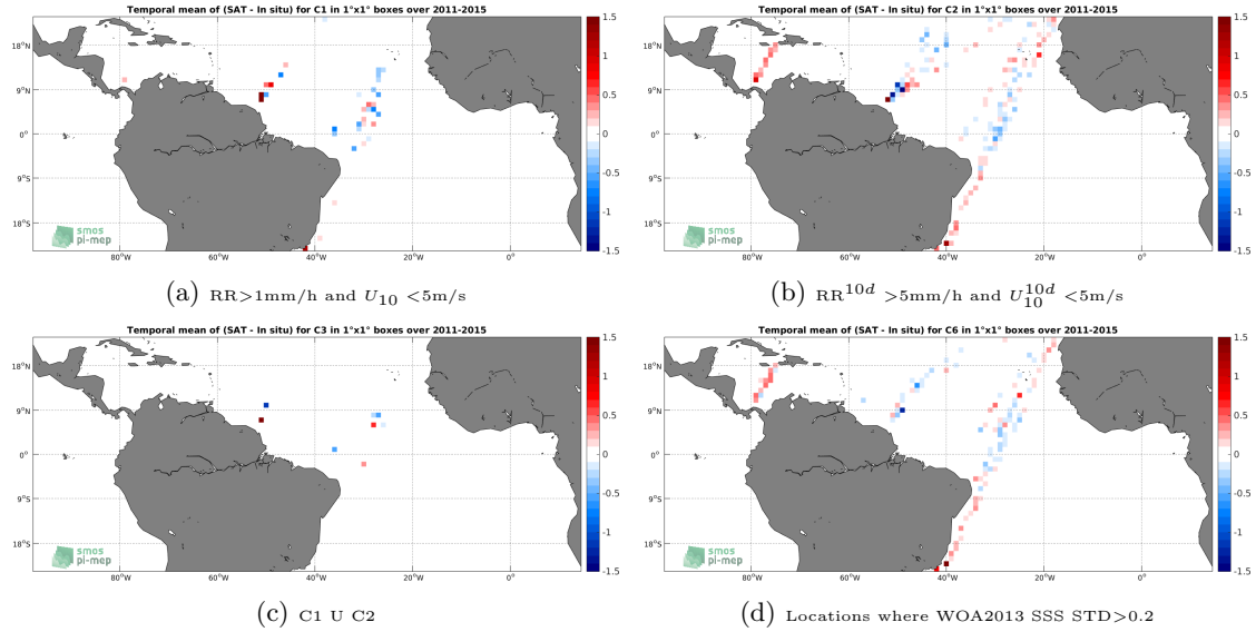
Figure 12: Temporal mean gridded over spatial boxes of size 1^\circ \times 1^\circ of \Delta SSS (Aquarius-L3-JPL-V5-7DAY-RUNNING - TSG-LEGOS-DM) for 4 different subdatasets corresponding to: RR > 1mm/h and U_{10} < 5\text{m/s} (a), RR^{10d} > 5\text{mm/h} and U_{10}^{10d} < 5\text{m/s} (b), C1 U C2 (c), Locations where WOA2013 SSS STD > 0.2 (d).
