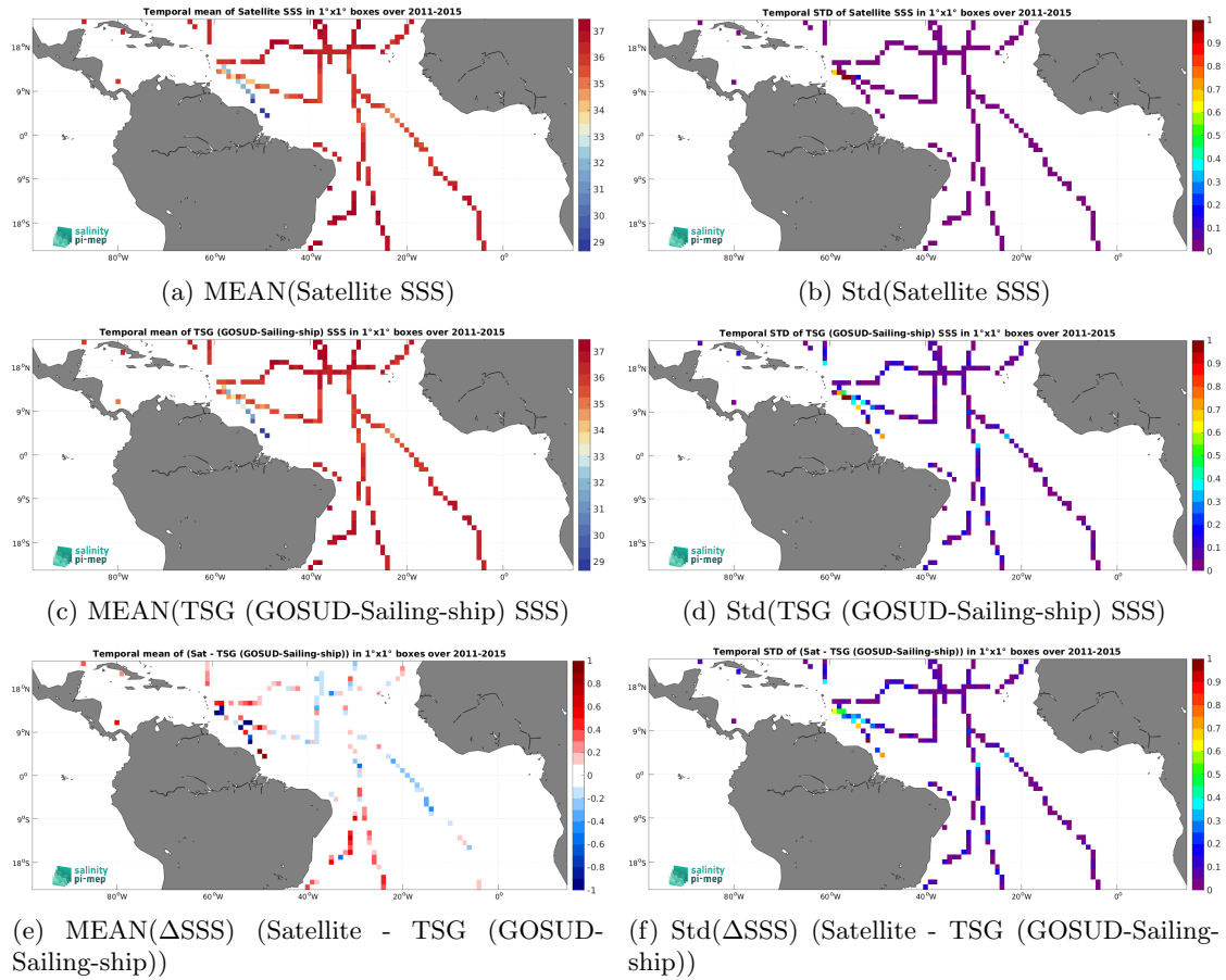
Figure 7: Temporal mean (left) and Std (right) of SSS from Aquarius SSS L3 CAP v5 - 7-Day running (JPL) (top), TSG (GOSUD-Sailing-ship) (middle), and of \Delta SSS (Satellite - TSG (GOSUD-Sailing-ship)). Only match-up pairs are used to generate these maps.
