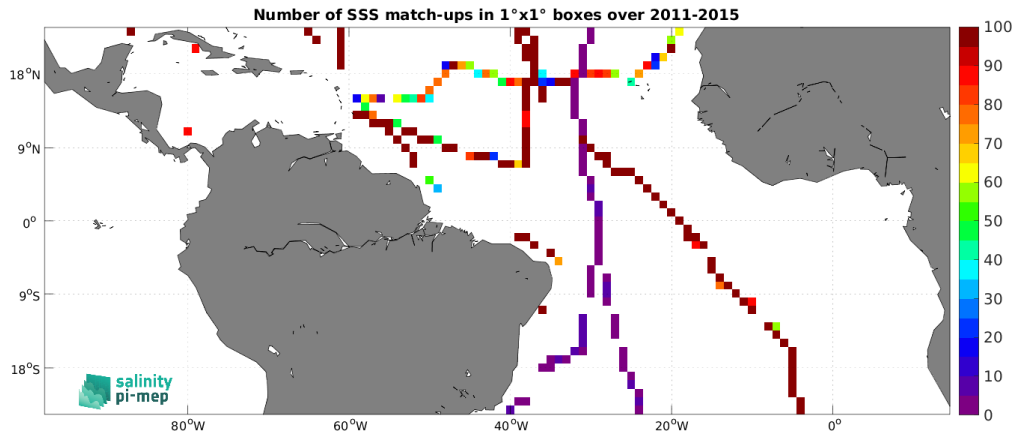
Figure 5: Number of SSS match-ups between TSG (GOSUD-Sailing-ship) SSS and the Aquarius SSS L3 CAP v5 - 7-Day running (JPL) SSS product for the Tropical Atlantic Ocean Pi-MEP region over 1^\circ \times 1^\circ boxes and for the full satellite product period.
