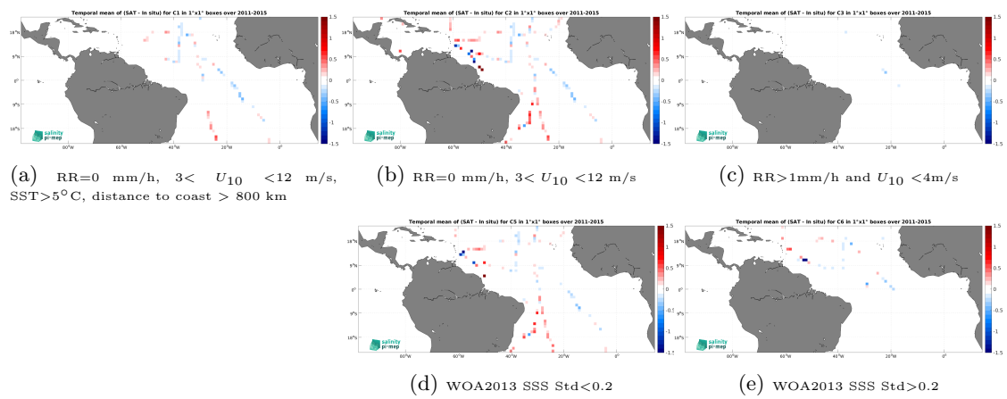
Figure 14: Temporal mean gridded over spatial boxes of size 1^\circ \times 1^\circ of \Delta\text{SSS} (Aquarius SSS L3 CAP v5 - 7-Day running (JPL) - TSG (GOSUD-Sailing-ship)) for 5 different subdatasets corresponding to:RR=0 mm/h, 3 < U_{10} < 12 m/s, SST >5^\circ\text{C} , distance to coast > 800 km (a), RR=0 mm/h, 3 < U_{10} < 12 m/s (b), RR >1 mm/h and U_{10} < 4 m/s (c), WOA2013 SSS Std <0.2 (d), WOA2013 SSS Std >0.2 (e).
