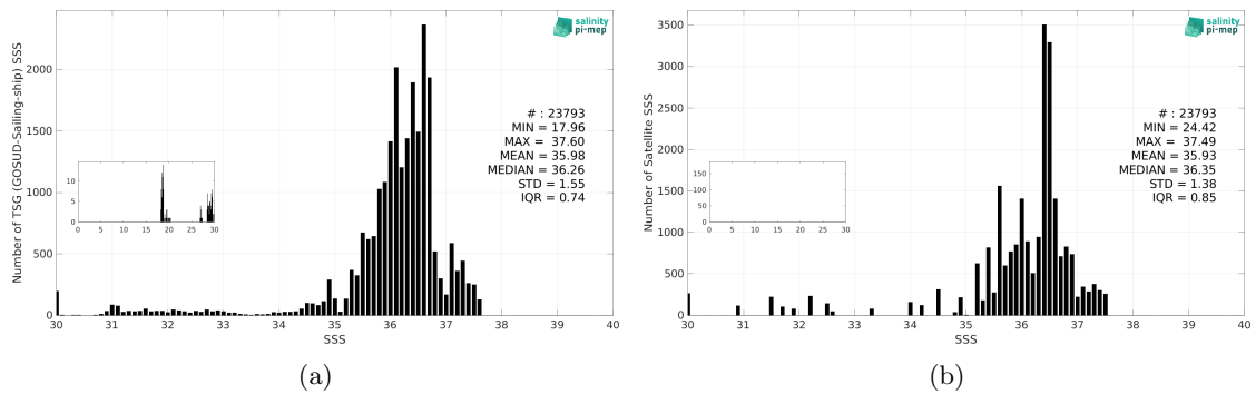
Figure 3: Histograms of SSS from TSG (GOSUD-Sailing-ship) (a) and Aquarius SSS L3 CAP v5 - 7-Day running (JPL) (b) considering all match-up pairs per bins of 0.1 over the Tropical Atlantic Ocean Pi-MEP region and for the full satellite product period.
