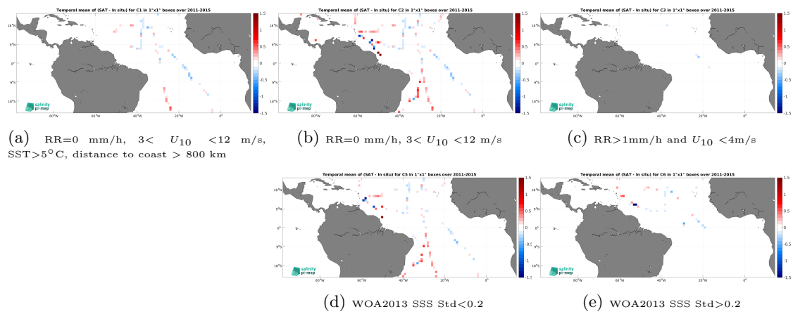
Figure 14: Temporal mean gridded over spatial boxes of size 1^\circ \times 1^\circ of \Delta\text{SSS} (Aquarius SSS L3 CAP v5 - 7-Day running (JPL) - TSG (GOSUD-Sailing-ship)) for 5 different subdatasets corresponding to:RR=0 mm/h, 3 < U_{10} < 12 m/s, SST >5^\circ\text{C} , distance to coast > 800 km (a), RR=0 mm/h, 3 < U_{10} < 12 m/s (b), RR >1 mm/h and U_{10} < 4 m/s (c), WOA2013 SSS Std <0.2 (d), WOA2013 SSS Std >0.2 (e).
