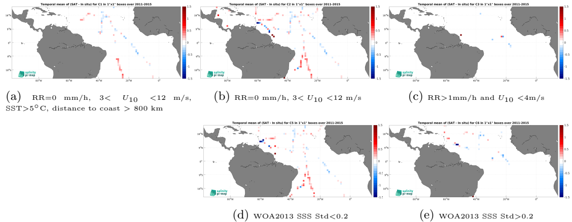
Figure 12: Temporal mean gridded over spatial boxes of size 1^{\circ}\times 1^{\circ} of \Delta SSS (Aquarius SSS L3 CAP v5 - 7-Day running (JPL) - TSG (GOSUD-Sailing-ship)) for 5 different subdatasets corresponding to:RR=0 mm/h, 3 < U_{10} < 12 m/s, SST > 5^{\circ}\text{C} , distance to coast > 800 km (a), RR=0 mm/h, 3 < U_{10} < 12 m/s (b), RR > 1 mm/h and U_{10} < 4 m/s (c), WOA2013 SSS Std < 0.2 (d), WOA2013 SSS Std > 0.2 (e).
