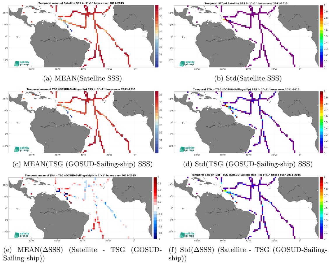
Figure 6: Temporal mean (left) and Std (right) of SSS from Aquarius SSS L3 CAP v5 - 7-Day running (JPL) (top), TSG (GOSUD-Sailing-ship) (middle), and of \Delta SSS (Satellite - TSG (GOSUD-Sailing-ship)). Only match-up pairs are used to generate these maps.
