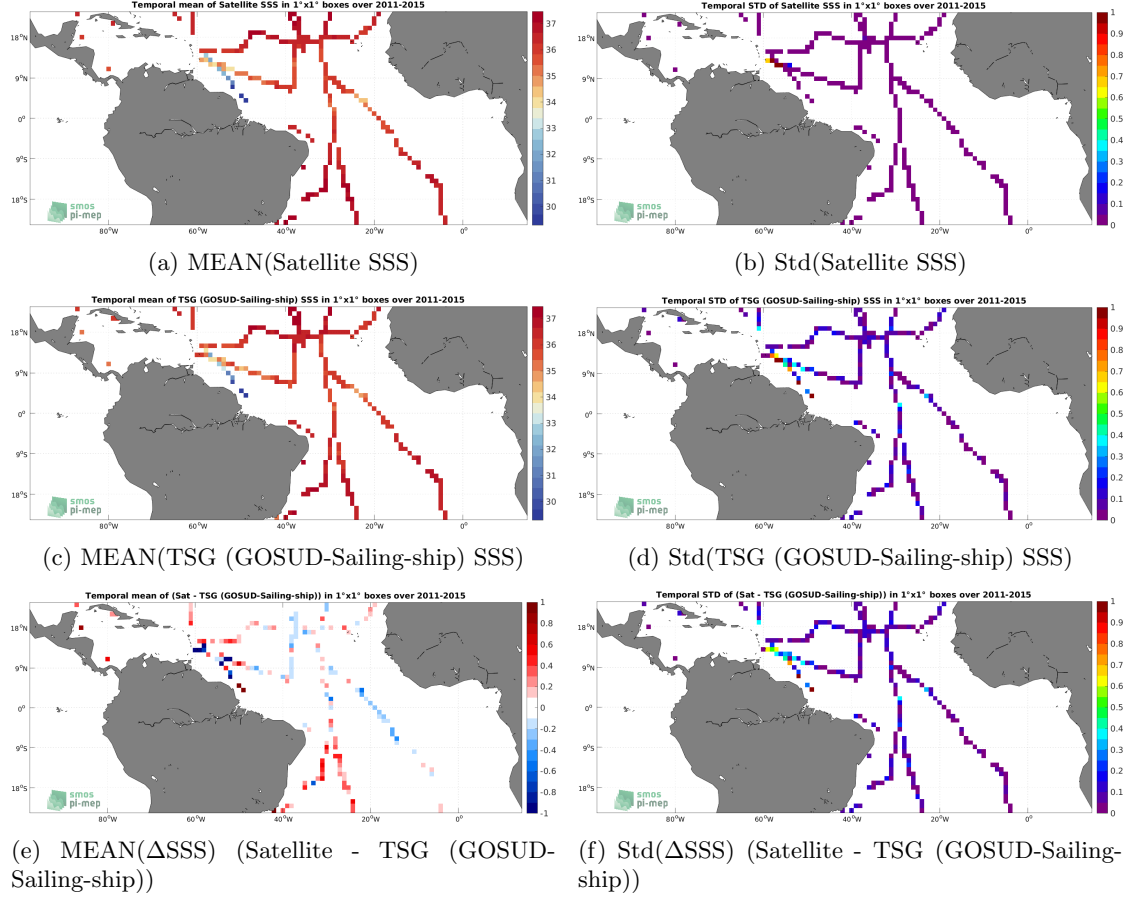
Figure 6: Temporal mean (left) and Std (right) of SSS from Aquarius SSS L3 CAP v5 - 7-Day running (JPL) (top), TSG (GOSUD-Sailing-ship) (middle), and of \Delta\text{SSS} (Satellite - TSG (GOSUD-Sailing-ship)). Only match-up pairs are used to generate these maps.
