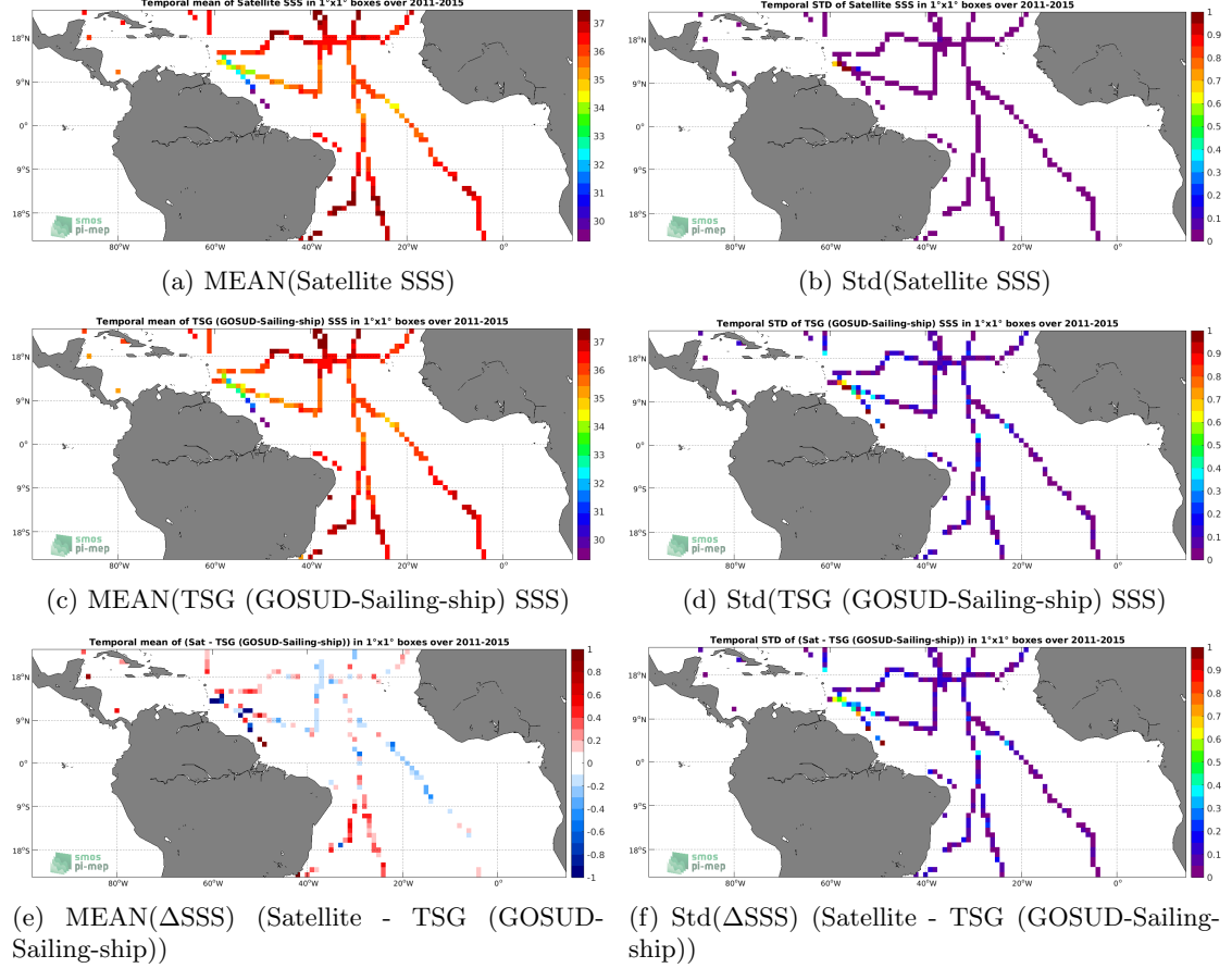
Figure 6: Temporal mean (left) and Std (right) of SSS from Aquarius SSS L3 CAP v5 - 7-Day running (JPL) (top), TSG (GOSUD-Sailing-ship) (middle), and of \Delta SSS (Satellite - TSG (GOSUD-Sailing-ship)). Only match-up pairs are used to generate these maps.
