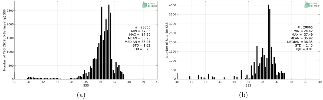
Figure 2: Histograms of SSS from TSG (GOSUD-Sailing-ship) (a) and Aquarius SSS L3 CAP v5 - 7-Day running (JPL) (b) considering all match-up pairs per bins of 0.1 over the Tropical Atlantic Ocean Pi-MEP region and for the full satellite product period.
