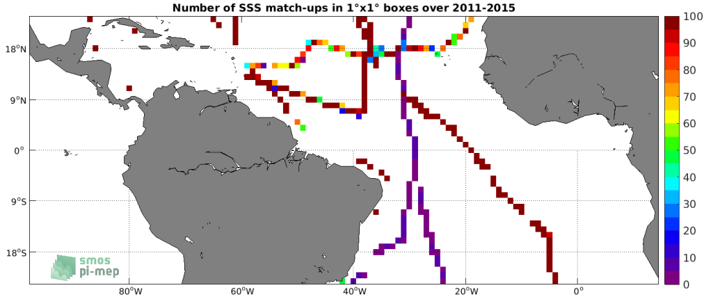
Figure 4: Number of SSS match-ups between TSG (GOSUD-Sailing-ship) SSS and the Aquarius SSS L3 CAP v5 - 7-Day running (JPL) SSS product for the Tropical Atlantic Ocean Pi-MEP region over 1^\circ \times 1^\circ boxes and for the full satellite product period.
