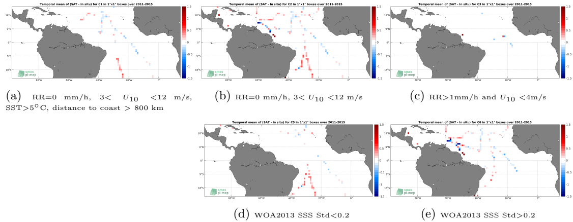
Figure 12: Temporal mean gridded over spatial boxes of size 1^\circ \times 1^\circ of \Delta SSS (Aquarius SSS L3 CAP v5 - 7-Day running (JPL) - TSG (GOSUD-Sailing-ship)) for 5 different subdatasets corresponding to:RR=0 mm/h, 3 < U_{10} < 12 m/s, SST >5^\circ\text{C} , distance to coast > 800 km (a), RR=0 mm/h, 3 < U_{10} < 12 m/s (b), RR >1 mm/h and U_{10} < 4 m/s (c), WOA2013 SSS Std <0.2 (d), WOA2013 SSS Std >0.2 (e).
