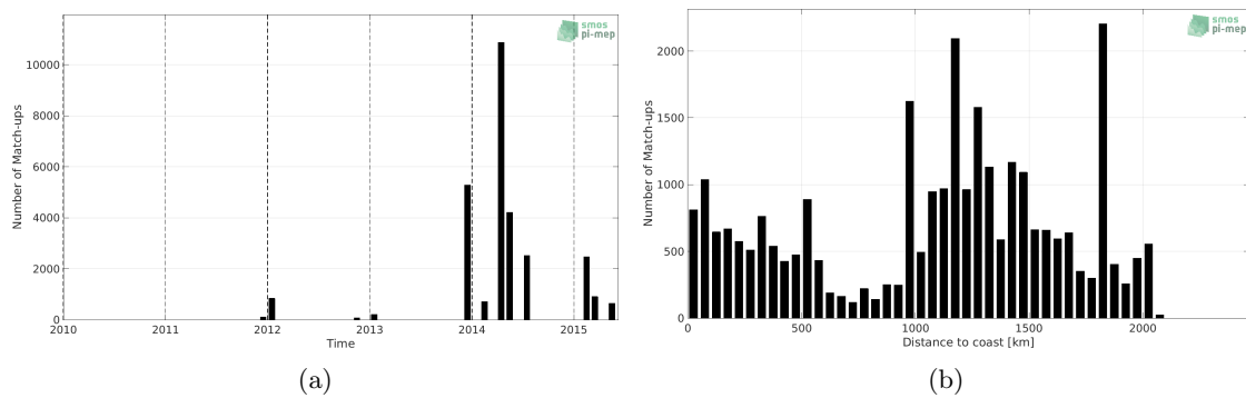
Figure 1: Number of match-ups between TSG (GOSUD-Sailing-ship) and Aquarius SSS L3 CAP v5 - 7-Day running (JPL) SSS as a function of time (a) and as function of the distance to coast (b) over the Tropical Atlantic Ocean Pi-MEP region and for the full satellite product period.
