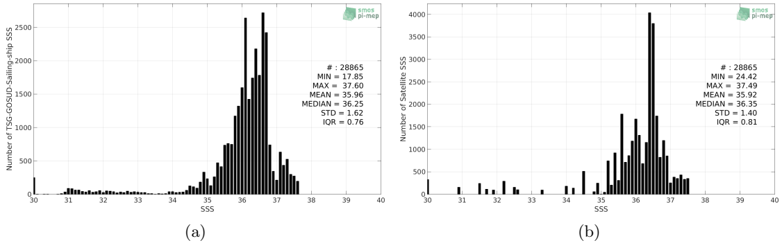
Figure 2: Histograms of SSS from TSG-GOSUD-Sailing-ship (a) and Aquarius-L3-JPL-V5-7DAY-RUNNING (b) considering all match-up pairs per bins of 0.1 over the Tropical Atlantic Ocean Pi-MEP region and for the full satellite product period.
