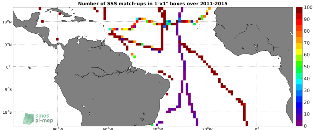
Figure 4: Number of SSS match-ups between TSG-GOSUD-Sailing-ship SSS and the Aquarius-L3-JPL-V5-7DAY-RUNNING SSS product for the Tropical Atlantic Ocean Pi-MEP region over 1^\circ \times 1^\circ boxes and for the full satellite product period.
