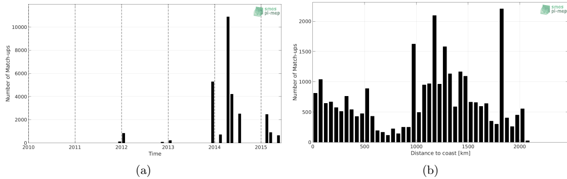
Figure 1: Number of match-ups between TSG-GOSUD-Sailing-ship and Aquarius-L3-JPL-V5-7DAY-RUNNING SSS as a function of time (a) and as function of the distance to coast (b) over the Tropical Atlantic Ocean Pi-MEP region and for the full satellite product period.
