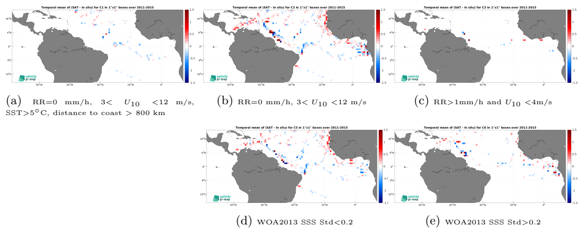
Figure 14: Temporal mean gridded over spatial boxes of size 1^\circ \times 1^\circ of \Delta SSS (Aquarius SSS L3 CAP v5 - 7-Day running (JPL) - TSG (GOSUD-Research-vessel)) for 5 different subdatasets corresponding to:RR=0 mm/h, 3 < U_{10} < 12 m/s, SST >5^\circ\text{C} , distance to coast > 800 km (a), RR=0 mm/h, 3 < U_{10} < 12 m/s (b), RR >1 mm/h and U_{10} < 4 m/s (c), WOA2013 SSS Std <0.2 (d), WOA2013 SSS Std >0.2 (e).
