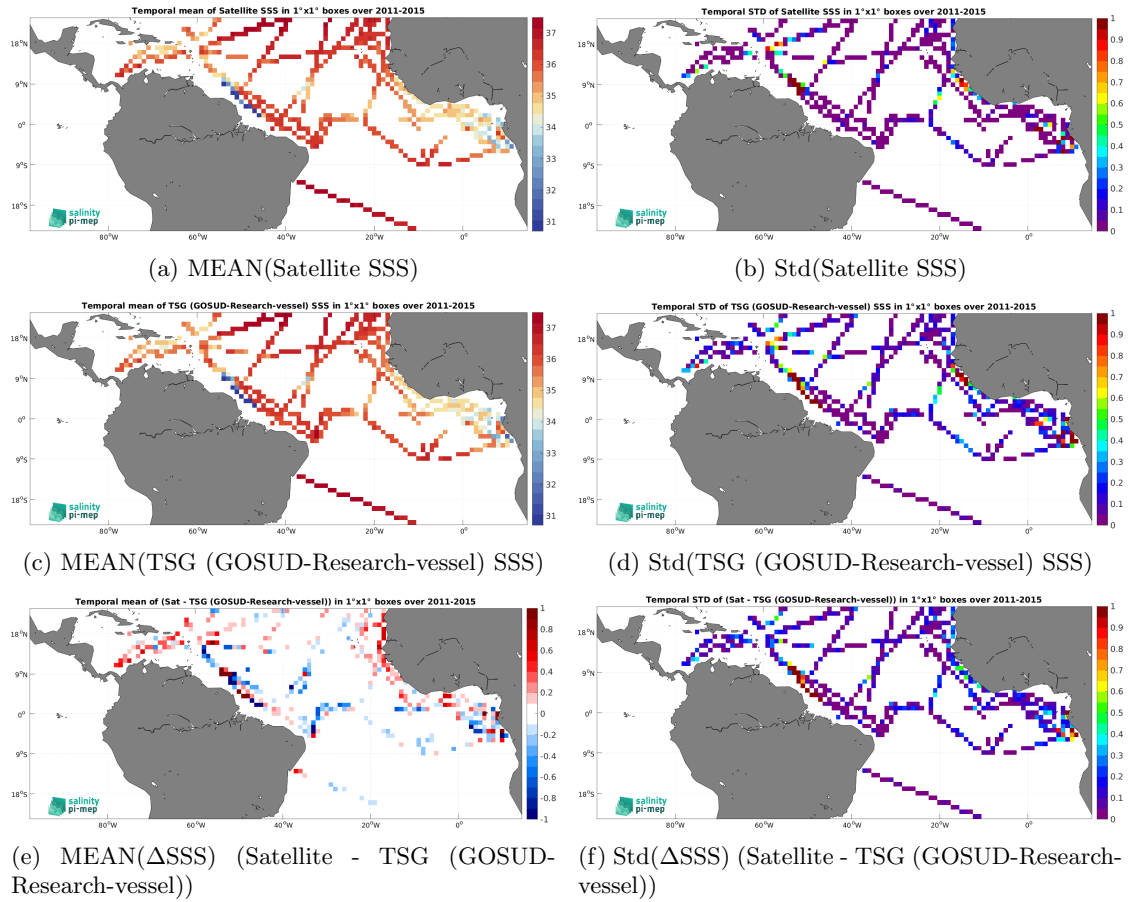
Figure 7: Temporal mean (left) and Std (right) of SSS from Aquarius SSS L3 CAP v5 - 7-Day running (JPL) (top), TSG (GOSUD-Research-vessel) (middle), and of \Delta SSS (Satellite - TSG (GOSUD-Research-vessel)). Only match-up pairs are used to generate these maps.
