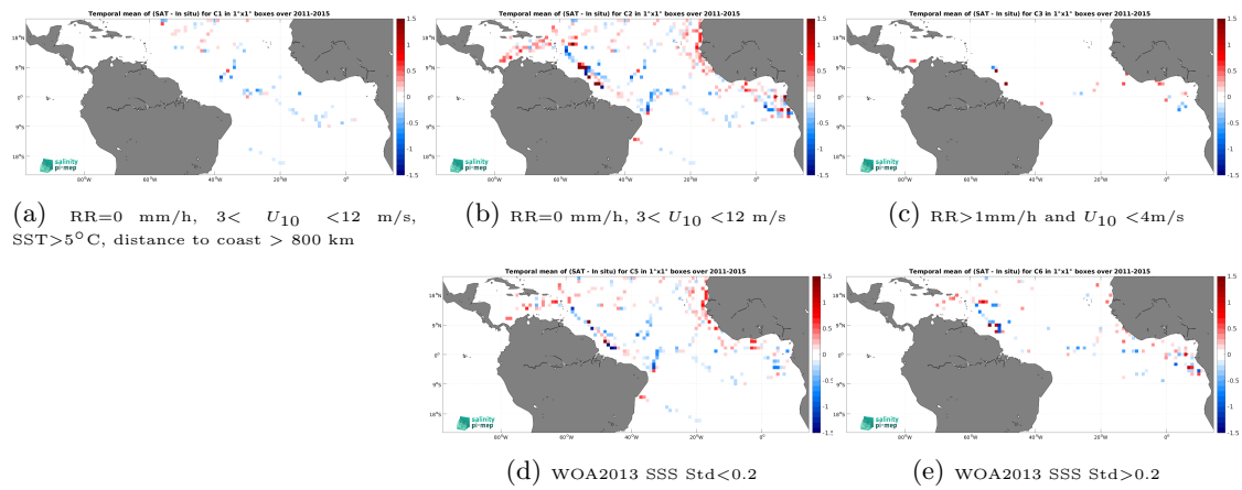
Figure 14: Temporal mean gridded over spatial boxes of size 1^\circ \times 1^\circ of \Delta\text{SSS} (Aquarius SSS L3 CAP v5 - 7-Day running (JPL) - TSG (GOSUD-Research-vessel)) for 5 different subdatasets corresponding to:RR=0 mm/h, 3 < U_{10} < 12 m/s, SST>5°C, distance to coast > 800 km (a), RR=0 mm/h, 3 < U_{10} < 12 m/s (b), RR>1mm/h and U_{10} < 4 m/s (c), WOA2013 SSS Std<0.2 (d), WOA2013 SSS Std>0.2 (e).
