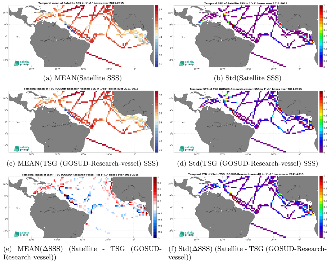
Figure 7: Temporal mean (left) and Std (right) of SSS from Aquarius SSS L3 CAP v5 - 7-Day running (JPL) (top), TSG (GOSUD-Research-vessel) (middle), and of \Delta SSS (Satellite - TSG (GOSUD-Research-vessel)). Only match-up pairs are used to generate these maps.
