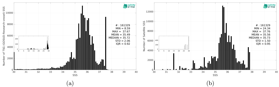
Figure 3: Histograms of SSS from TSG (GOSUD-Research-vessel) (a) and Aquarius SSS L3 CAP v5 - 7-Day running (JPL) (b) considering all match-up pairs per bins of 0.1 over the Tropical Atlantic Ocean Pi-MEP region and for the full satellite product period.
