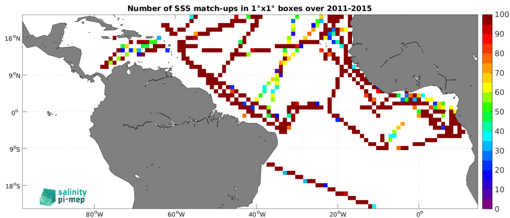
Figure 5: Number of SSS match-ups between TSG (GOSUD-Research-vessel) SSS and the Aquarius SSS L3 CAP v5 - 7-Day running (JPL) SSS product for the Tropical Atlantic Ocean Pi-MEP region over 1^\circ \times 1^\circ boxes and for the full satellite product period.
