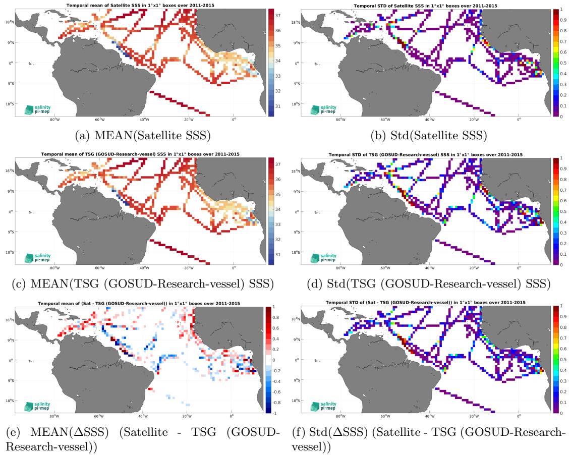
Figure 6: Temporal mean (left) and Std (right) of SSS from Aquarius SSS L3 CAP v5 - 7-Day running (JPL) (top), TSG (GOSUD-Research-vessel) (middle), and of \Delta SSS (Satellite - TSG (GOSUD-Research-vessel)). Only match-up pairs are used to generate these maps.
