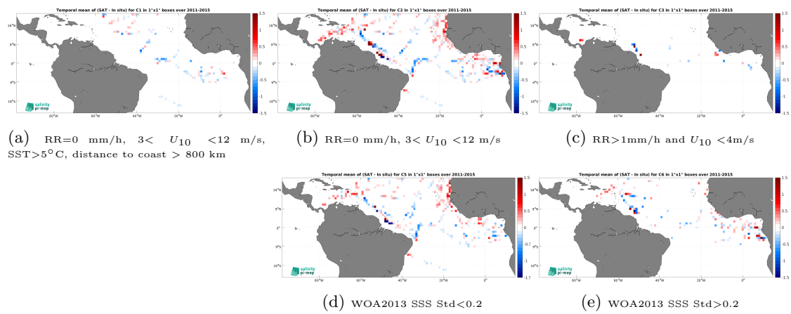
Figure 12: Temporal mean gridded over spatial boxes of size 1^\circ \times 1^\circ of \Delta SSS (Aquarius SSS L3 CAP v5 - 7-Day running (JPL) - TSG (GOSUD-Research-vessel)) for 5 different subdatasets corresponding to:RR=0 mm/h, 3 < U_{10} < 12 m/s, SST >5^\circ\text{C} , distance to coast > 800 km (a), RR=0 mm/h, 3 < U_{10} < 12 m/s (b), RR >1 mm/h and U_{10} < 4 m/s (c), WOA2013 SSS Std <0.2 (d), WOA2013 SSS Std >0.2 (e).
