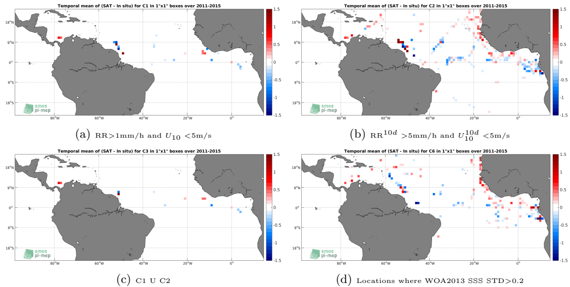
Figure 12: Temporal mean gridded over spatial boxes of size 1^\circ \times 1^\circ of \Delta SSS (Aquarius-L3-JPL-V5-7DAY-RUNNING - TSG-GOSUD-Research-vessel) for 4 different subdatasets corresponding to: RR > 1\text{mm/h} and U_{10} < 5\text{m/s} (a), RR^{10d} > 5\text{mm/h} and U_{10}^{10d} < 5\text{m/s} (b), C1 U C2 (c), Locations where WOA2013 SSS STD > 0.2 (d).
