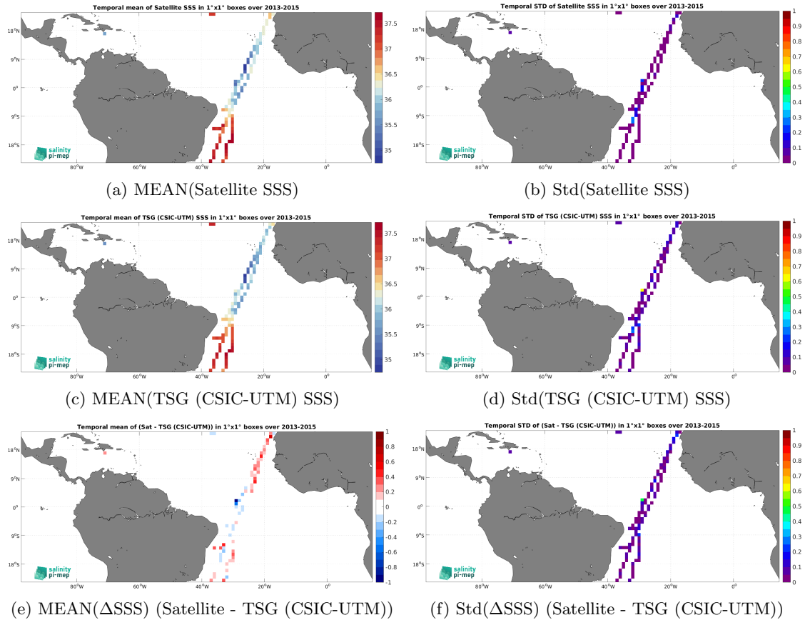
Figure 7: Temporal mean (left) and Std (right) of SSS from Aquarius SSS L3 CAP v5 - 7-Day running (JPL) (top), TSG (CSIC-UTM) (middle), and of \Delta SSS (Satellite - TSG (CSIC-UTM)). Only match-up pairs are used to generate these maps.
