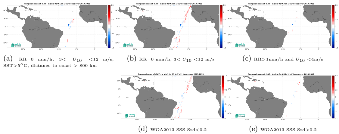
Figure 14: Temporal mean gridded over spatial boxes of size 1^\circ \times 1^\circ of \Delta SSS (Aquarius SSS L3 CAP v5 - 7-Day running (JPL) - TSG (CSIC-UTM)) for 5 different subdatasets corresponding to:RR=0 mm/h, 3 < U_{10} < 12 m/s, SST >5^\circ\text{C} , distance to coast > 800 km (a), RR=0 mm/h, 3 < U_{10} < 12 m/s (b), RR >1 mm/h and U_{10} < 4 m/s (c), WOA2013 SSS Std <0.2 (d), WOA2013 SSS Std >0.2 (e).
