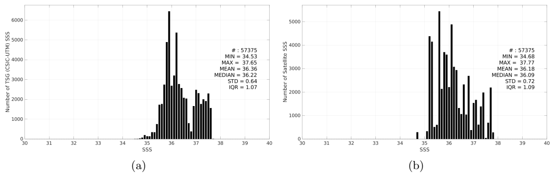
Figure 3: Histograms of SSS from TSG (CSIC-UTM) (a) and Aquarius SSS L3 CAP v5 - 7-Day running (JPL) (b) considering all match-up pairs per bins of 0.1 over the Tropical Atlantic Ocean Pi-MEP region and for the full satellite product period.
