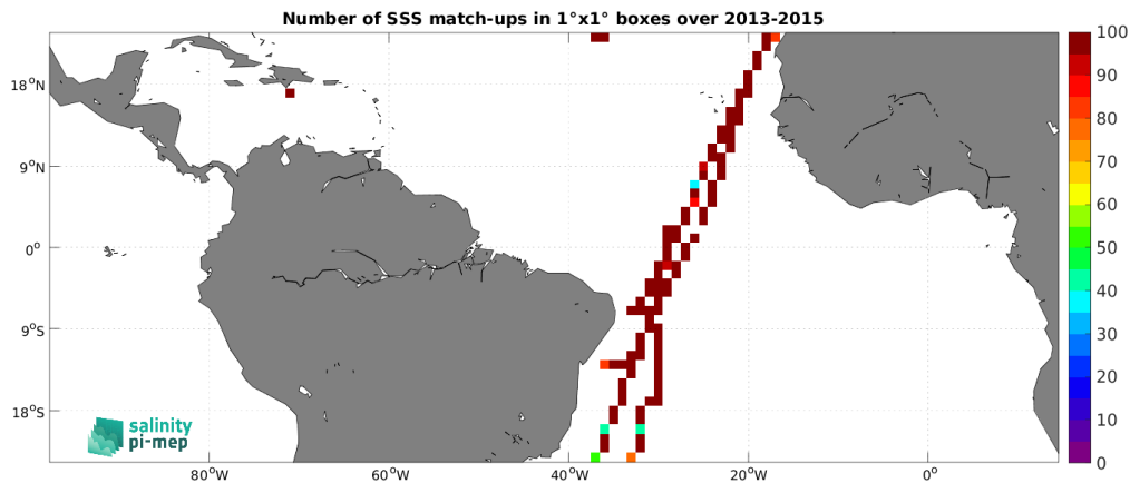
Figure 5: Number of SSS match-ups between TSG (CSIC-UTM) SSS and the Aquarius SSS L3 CAP v5 - 7-Day running (JPL) SSS product for the Tropical Atlantic Ocean Pi-MEP region over 1^\circ \times 1^\circ boxes and for the full satellite product period.
