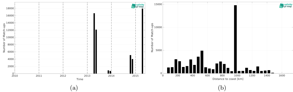
Figure 2: Number of match-ups between TSG (CSIC-UTM) and Aquarius SSS L3 CAP v5 - 7-Day running (JPL) SSS as a function of time (a) and as function of the distance to coast (b) over the Tropical Atlantic Ocean Pi-MEP region and for the full satellite product period.
