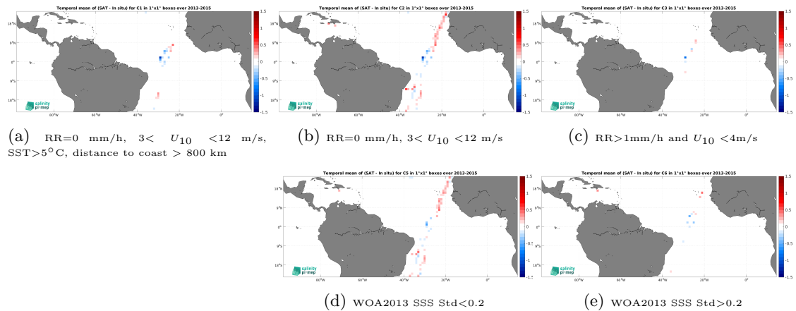
Figure 12: Temporal mean gridded over spatial boxes of size 1^\circ \times 1^\circ of \Delta SSS (Aquarius SSS L3 CAP v5 - 7-Day running (JPL) - TSG (CSIC-UTM)) for 5 different subdatasets corresponding to:RR=0 mm/h, 3 < U_{10} < 12 m/s, SST >5^\circ\text{C} , distance to coast > 800 km (a), RR=0 mm/h, 3 < U_{10} < 12 m/s (b), RR >1 mm/h and U_{10} < 4 m/s (c), WOA2013 SSS Std <0.2 (d), WOA2013 SSS Std >0.2 (e).
