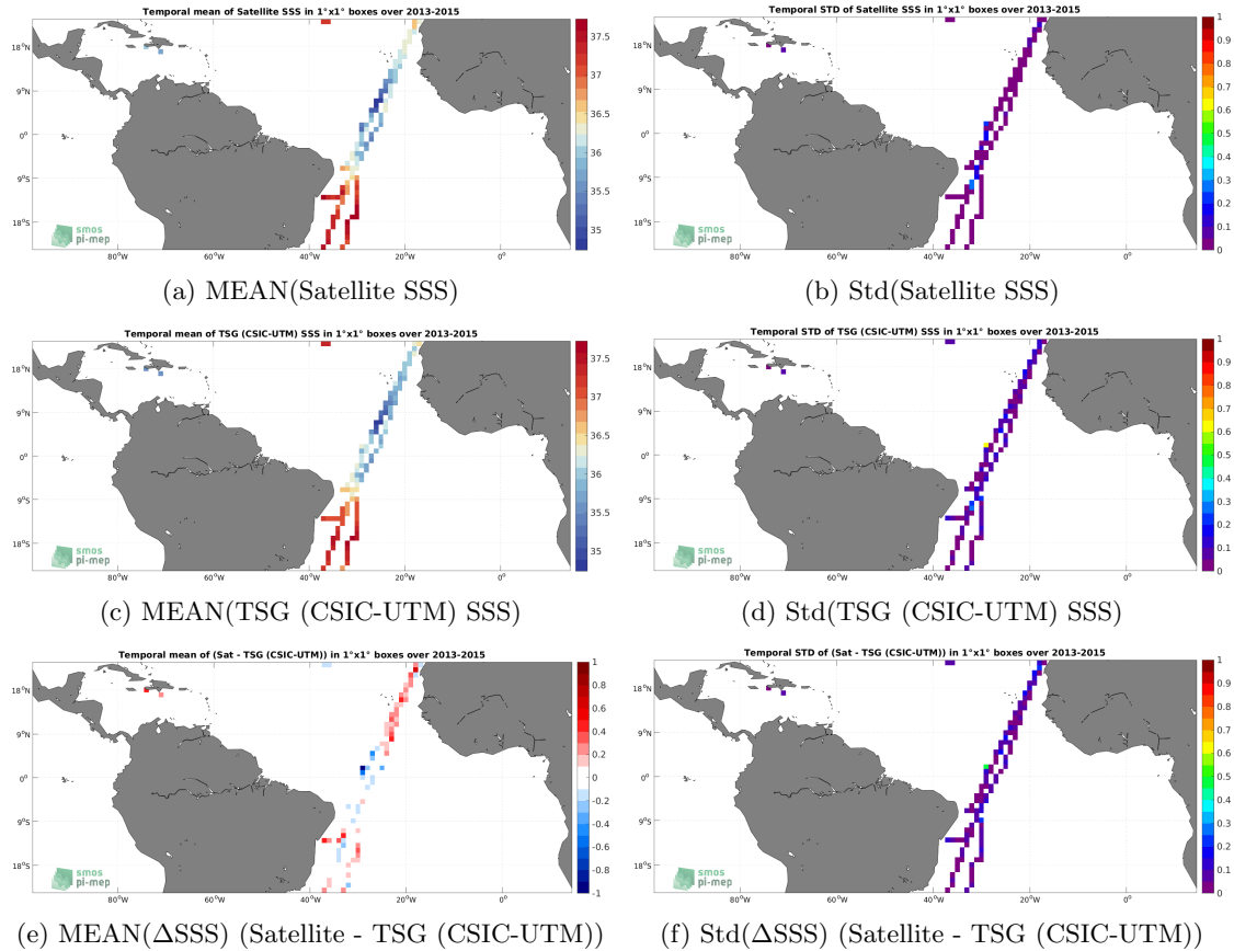
Figure 6: Temporal mean (left) and Std (right) of SSS from Aquarius SSS L3 CAP v5 - 7-Day running (JPL) (top), TSG (CSIC-UTM) (middle), and of \Delta SSS (Satellite - TSG (CSIC-UTM)). Only match-up pairs are used to generate these maps.
