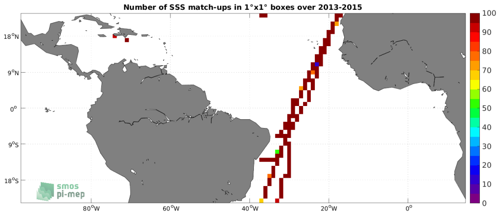
Figure 4: Number of SSS match-ups between TSG (CSIC-UTM) SSS and the Aquarius SSS L3 CAP v5 - 7-Day running (JPL) SSS product for the Tropical Atlantic Ocean Pi-MEP region over 1^\circ \times 1^\circ boxes and for the full satellite product period.
