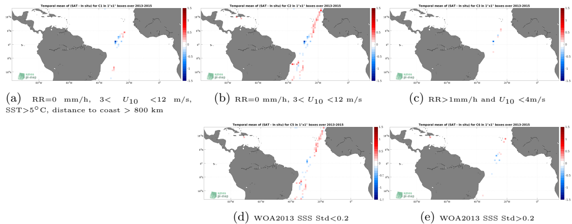
Figure 12: Temporal mean gridded over spatial boxes of size 1^\circ \times 1^\circ of \Delta\text{SSS} (Aquarius SSS L3 CAP v5 - 7-Day running (JPL) - TSG (CSIC-UTM)) for 5 different subdatasets corresponding to:RR=0 mm/h, 3 < U_{10} < 12 m/s, SST >5^\circ\text{C} , distance to coast > 800 km (a), RR=0 mm/h, 3 < U_{10} < 12 m/s (b), RR >1 mm/h and U_{10} < 4 m/s (c), WOA2013 SSS Std <0.2 (d), WOA2013 SSS Std >0.2 (e).
