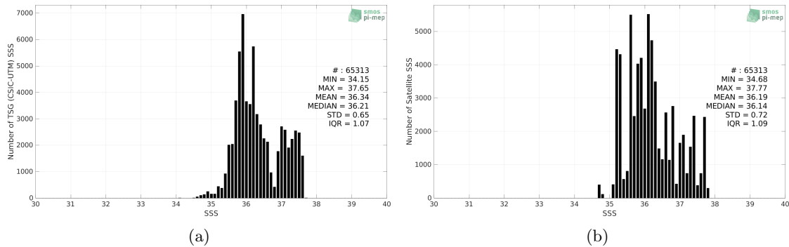
Figure 2: Histograms of SSS from TSG (CSIC-UTM) (a) and Aquarius SSS L3 CAP v5 - 7-Day running (JPL) (b) considering all match-up pairs per bins of 0.1 over the Tropical Atlantic Ocean Pi-MEP region and for the full satellite product period.
