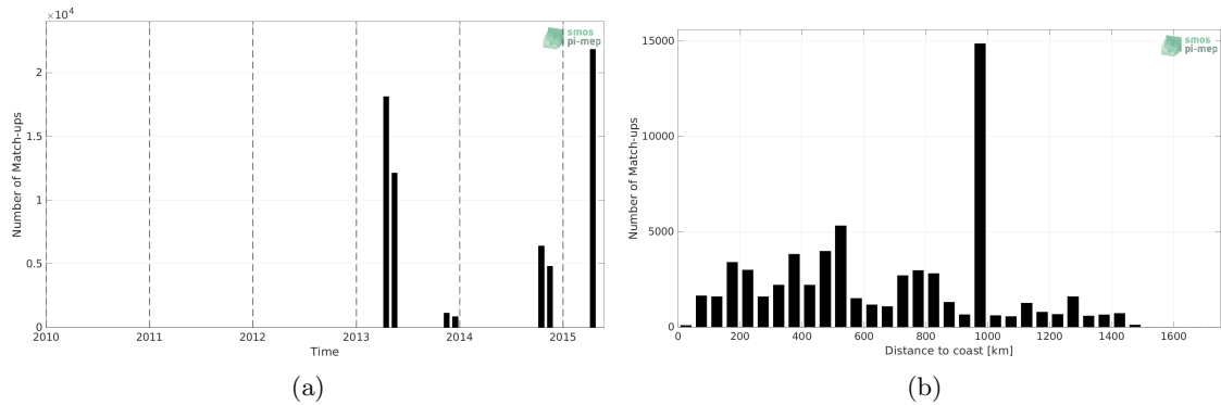
Figure 1: Number of match-ups between TSG (CSIC-UTM) and Aquarius SSS L3 CAP v5 - 7-Day running (JPL) SSS as a function of time (a) and as function of the distance to coast (b) over the Tropical Atlantic Ocean Pi-MEP region and for the full satellite product period.
