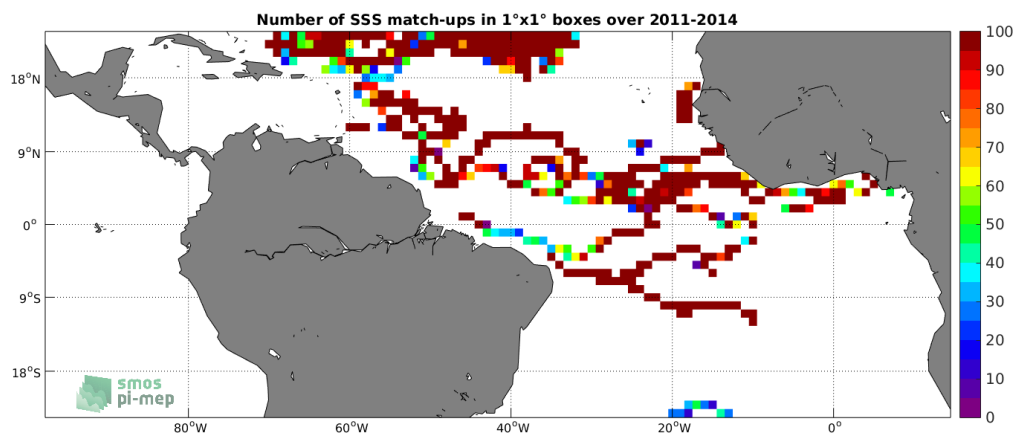
Figure 3: Number of SSS match-ups between Surface drifters SSS and the Aquarius-L3-JPL-V5-7DAY-RUNNING SSS product for the Tropical Atlantic Ocean Pi-MEP region over 1^\circ \times 1^\circ boxes and for the full satellite product period.
