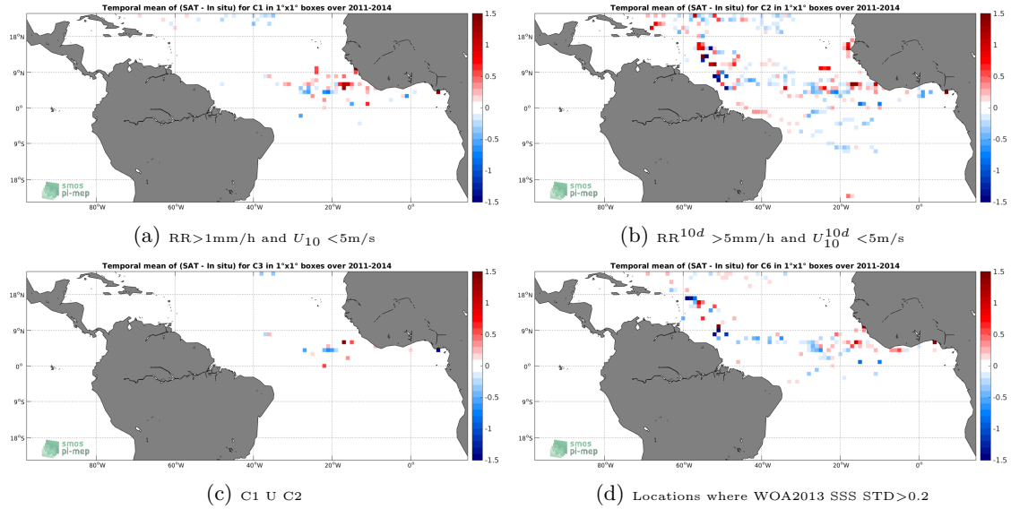
Figure 11: Temporal mean gridded over spatial boxes of size 1^\circ \times 1^\circ of \Delta SSS (Aquarius-L3-JPL-V5-7DAY-RUNNING - Surface drifters) for 4 different subdatasets corresponding to: RR > 1mm/h and U_{10} < 5\text{m/s} (a), RR^{10d} > 5\text{mm/h} and U_{10}^{10d} < 5\text{m/s} (b), C1 U C2 (c), Locations where WOA2013 SSS STD > 0.2 (d).
