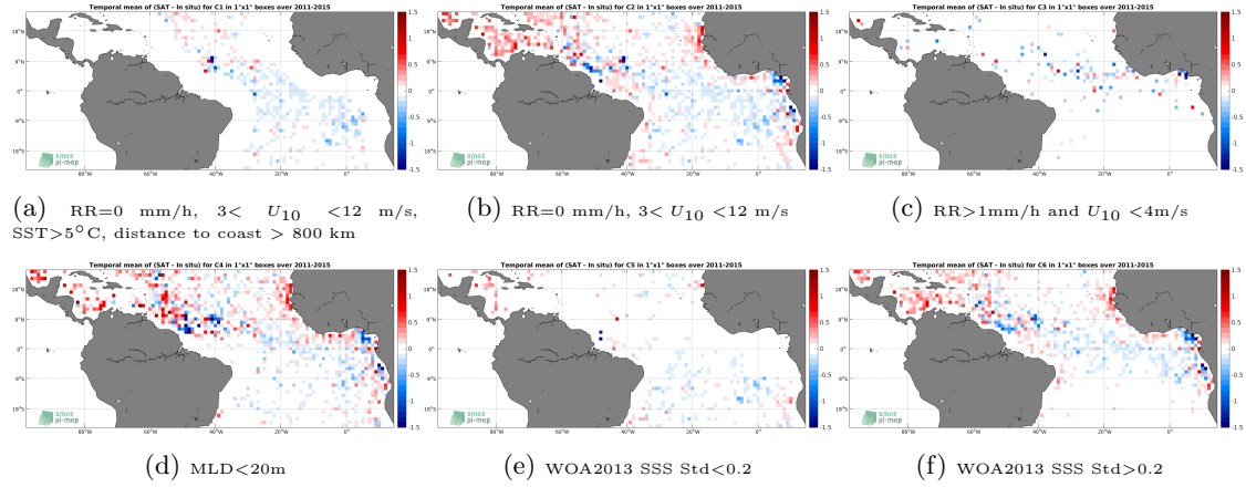
Figure 12: Temporal mean gridded over spatial boxes of size 1^\circ \times 1^\circ of \Delta SSS (Aquarius-L3-JPL-V5-7DAY-RUNNING - Argo) for 6 different subdatasets corresponding to: RR=0 mm/h, 3 < U_{10} < 12 m/s, SST > 5^\circ C , distance to coast > 800 km (a), RR=0 mm/h, 3 < U_{10} < 12 m/s (b), RR > 1 mm/h and U_{10} < 4 m/s (c), MLD < 20 m (d), WOA2013 SSS Std < 0.2 (e), WOA2013 SSS Std > 0.2 (f).
