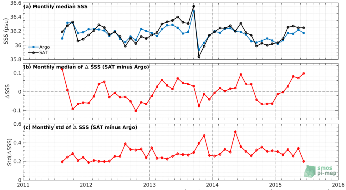
Figure 7: Time series of the monthly median SSS (top), median of \Delta\text{SSS} (Satellite - Argo) and Std of \Delta\text{SSS} (Satellite - Argo) over the Tropical Atlantic Ocean Pi-MEP region considering all match-ups collected by the Pi-MEP.
