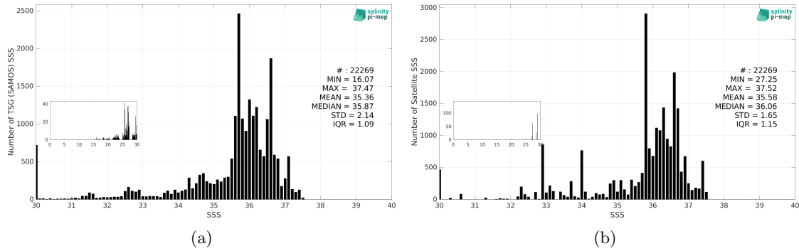
Figure 3: Histograms of SSS from TSG (SAMOS) (a) and Aquarius SSS L3 CAP v5 - Monthly (JPL) (b) considering all match-up pairs per bins of 0.1 over the Tropical Atlantic Ocean Pi-MEP region and for the full satellite product period.
