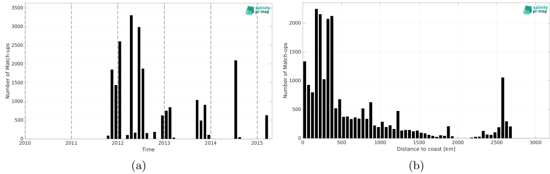
Figure 2: Number of match-ups between TSG (SAMOS) and Aquarius SSS L3 CAP v5 - Monthly (JPL) SSS as a function of time (a) and as function of the distance to coast (b) over the Tropical Atlantic Ocean Pi-MEP region and for the full satellite product period.
