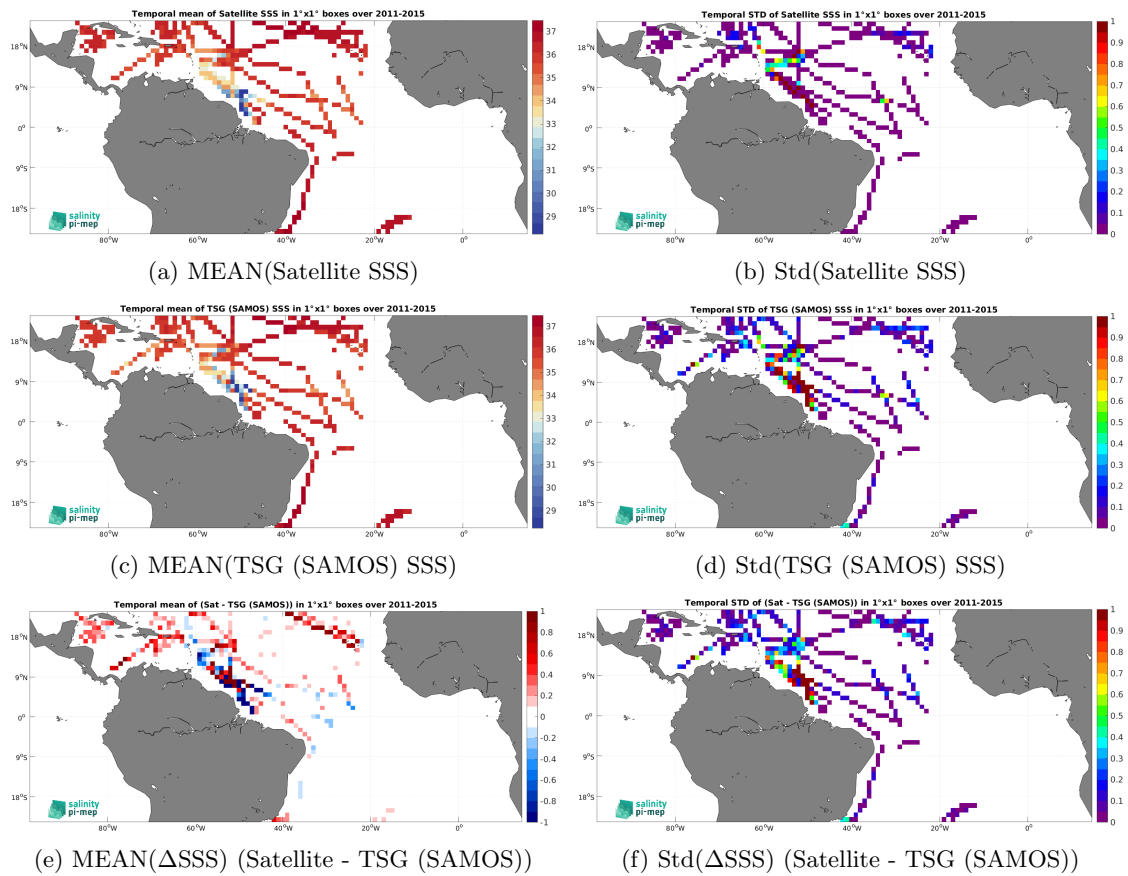
Figure 7: Temporal mean (left) and Std (right) of SSS from Aquarius SSS L3 CAP v5 - Monthly (JPL) (top), TSG (SAMOS) (middle), and of \Delta SSS (Satellite - TSG (SAMOS)). Only match-up pairs are used to generate these maps.
