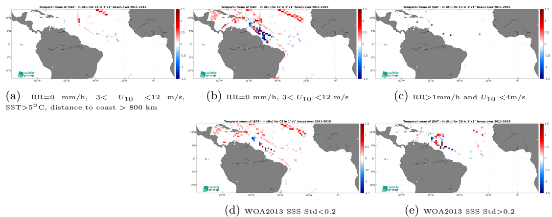
Figure 14: Temporal mean gridded over spatial boxes of size 1^\circ \times 1^\circ of \Delta SSS (Aquarius SSS L3 CAP v5 - Monthly (JPL) - TSG (SAMOS)) for 5 different subdatasets corresponding to:RR=0 mm/h, 3 < U_{10} < 12 m/s, SST >5^\circ\text{C} , distance to coast > 800 km (a), RR=0 mm/h, 3 < U_{10} < 12 m/s (b), RR >1 mm/h and U_{10} < 4 m/s (c), WOA2013 SSS Std <0.2 (d), WOA2013 SSS Std >0.2 (e).
