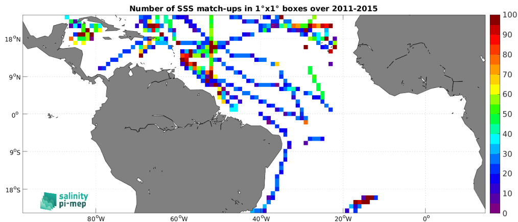
Figure 5: Number of SSS match-ups between TSG (SAMOS) SSS and the Aquarius SSS L3 CAP v5 - Monthly (JPL) SSS product for the Tropical Atlantic Ocean Pi-MEP region over 1^\circ \times 1^\circ boxes and for the full satellite product period.
