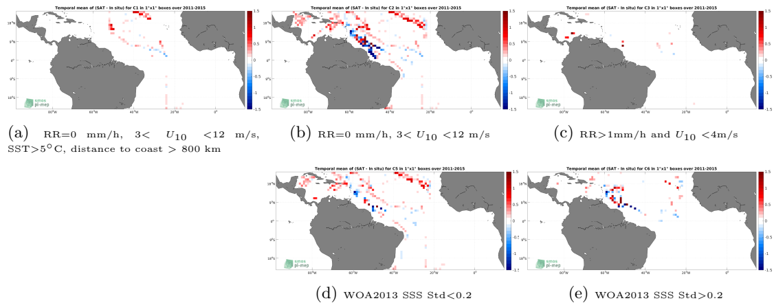
Figure 12: Temporal mean gridded over spatial boxes of size 1^\circ \times 1^\circ of \Delta\text{SSS} (Aquarius SSS L3 CAP v5 - Monthly (JPL) - TSG (SAMOS)) for 5 different subdatasets corresponding to:RR=0 mm/h, 3 < U_{10} < 12 m/s, SST >5^\circ\text{C} , distance to coast > 800 km (a), RR=0 mm/h, 3 < U_{10} < 12 m/s (b), RR >1 mm/h and U_{10} < 4 m/s (c), WOA2013 SSS Std <0.2 (d), WOA2013 SSS Std >0.2 (e).
