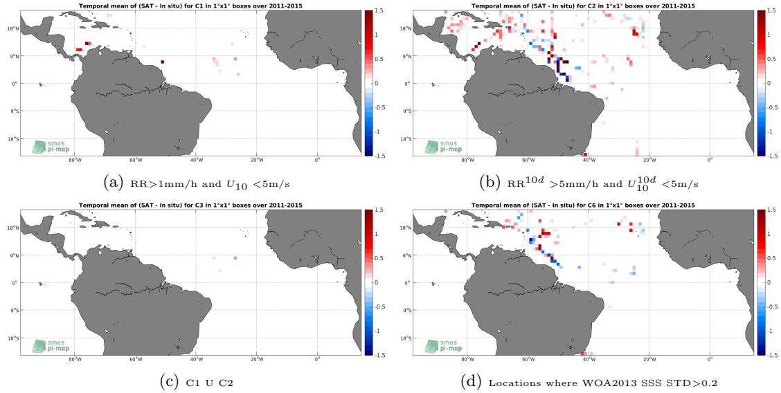
Figure 12: Temporal mean gridded over spatial boxes of size 1^\circ \times 1^\circ of \Delta SSS (Aquarius-L3-JPL-V5-MONTHLY - TSG-SAMOS) for 4 different subdatasets corresponding to:RR >1\text{mm/h} and U_{10} < 5\text{m/s} (a), RR^{10d} > 5\text{mm/h} and U_{10}^{10d} < 5\text{m/s} (b), C1 U C2 (c),Locations where WOA2013 SSS STD >0.2 (d).
