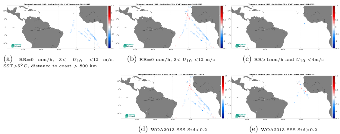
Figure 14: Temporal mean gridded over spatial boxes of size 1^\circ \times 1^\circ of \Delta SSS (Aquarius SSS L3 CAP v5 - Monthly (JPL) - TSG (Polarstern)) for 5 different subdatasets corresponding to:RR=0 mm/h, 3 < U_{10} < 12 m/s, SST > 5°C, distance to coast > 800 km (a), RR=0 mm/h, 3 < U_{10} < 12 m/s (b), RR > 1mm/h and U_{10} < 4 m/s (c), WOA2013 SSS Std < 0.2 (d), WOA2013 SSS Std > 0.2 (e).
