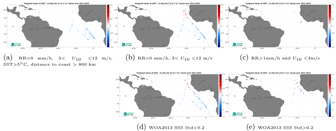
Figure 12: Temporal mean gridded over spatial boxes of size 1^\circ \times 1^\circ of \Delta\text{SSS} (Aquarius SSS L3 CAP v5 - Monthly (JPL) - TSG (Polarstern)) for 5 different subdatasets corresponding to:RR=0 mm/h, 3 < U_{10} < 12 m/s, SST >5^\circ\text{C} , distance to coast > 800 km (a), RR=0 mm/h, 3 < U_{10} < 12 m/s (b), RR >1 mm/h and U_{10} < 4 m/s (c), WOA2013 SSS Std <0.2 (d), WOA2013 SSS Std >0.2 (e).
