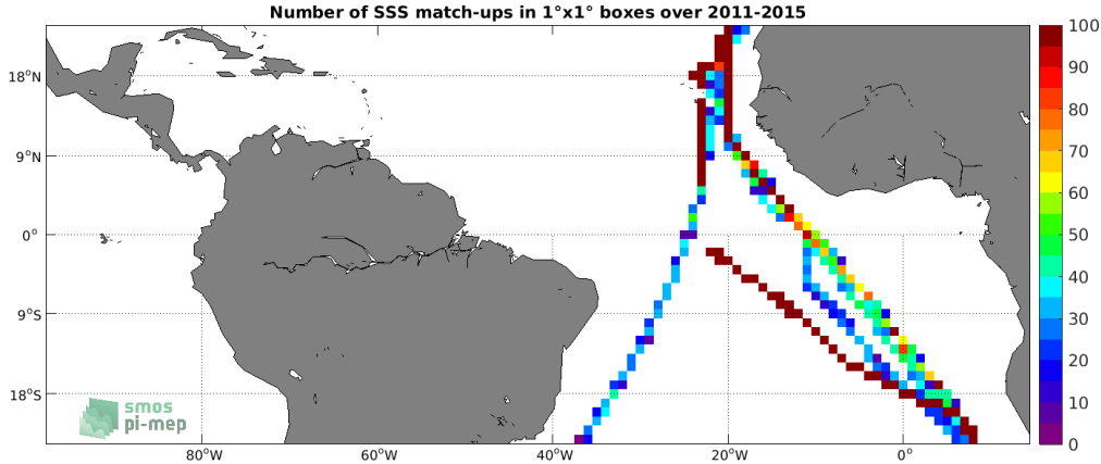
Figure 4: Number of SSS match-ups between TSG (Polarstern) SSS and the Aquarius SSS L3 CAP v5 - Monthly (JPL) SSS product for the Tropical Atlantic Ocean Pi-MEP region over 1^\circ \times 1^\circ boxes and for the full satellite product period.
