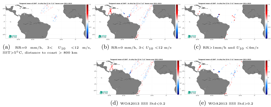
Figure 14: Temporal mean gridded over spatial boxes of size 1^\circ \times 1^\circ of \Delta SSS (Aquarius SSS L3 CAP v5 - Monthly (JPL) - TSG (LEGOS-DM)) for 5 different subdatasets corresponding to:RR=0 mm/h, 3 < U_{10} < 12 m/s, SST >5^\circ\text{C} , distance to coast > 800 km (a), RR=0 mm/h, 3 < U_{10} < 12 m/s (b), RR >1 mm/h and U_{10} < 4 m/s (c), WOA2013 SSS Std <0.2 (d), WOA2013 SSS Std >0.2 (e).
