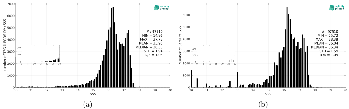
Figure 3: Histograms of SSS from TSG (LEGOS-DM) (a) and Aquarius SSS L3 CAP v5 - Monthly (JPL) (b) considering all match-up pairs per bins of 0.1 over the Tropical Atlantic Ocean Pi-MEP region and for the full satellite product period.
