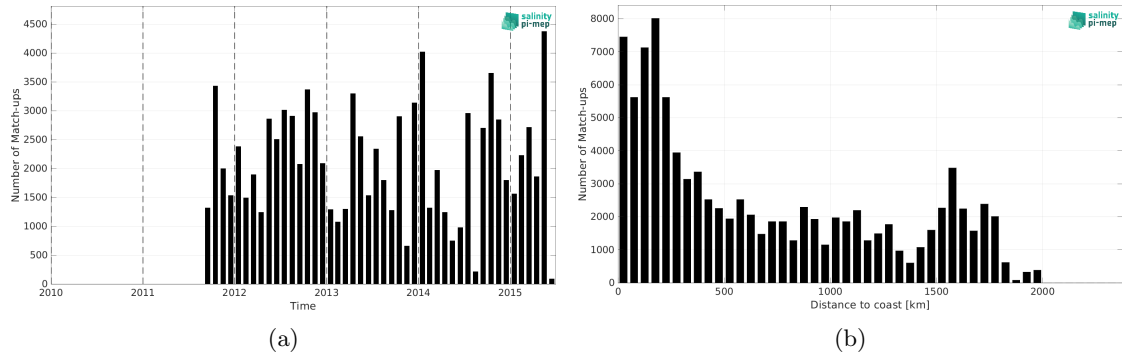
Figure 2: Number of match-ups between TSG (LEGOS-DM) and Aquarius SSS L3 CAP v5 - Monthly (JPL) SSS as a function of time (a) and as function of the distance to coast (b) over the Tropical Atlantic Ocean Pi-MEP region and for the full satellite product period.
