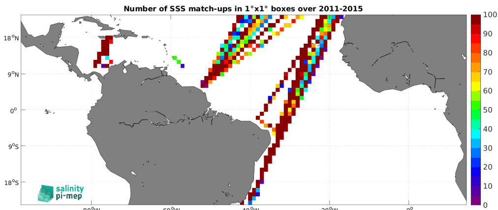
Figure 5: Number of SSS match-ups between TSG (LEGOS-DM) SSS and the Aquarius SSS L3 CAP v5 - Monthly (JPL) SSS product for the Tropical Atlantic Ocean Pi-MEP region over 1^\circ \times 1^\circ boxes and for the full satellite product period.
