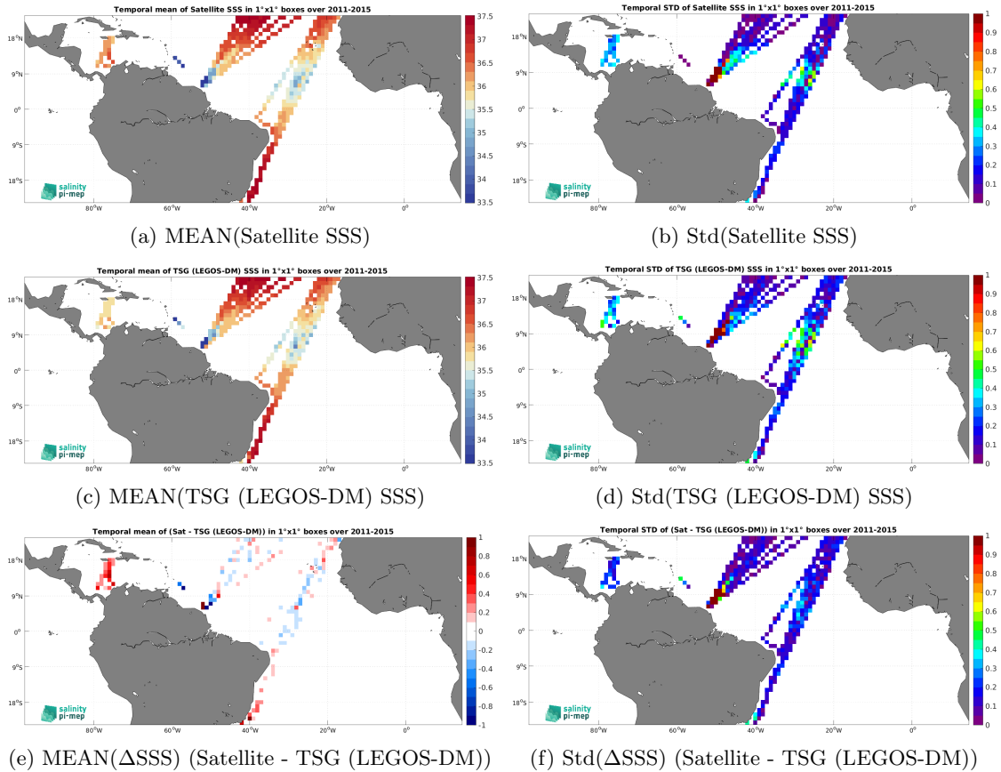
Figure 7: Temporal mean (left) and Std (right) of SSS from Aquarius SSS L3 CAP v5 - Monthly (JPL) (top), TSG (LEGOS-DM) (middle), and of \Delta SSS (Satellite - TSG (LEGOS-DM)). Only match-up pairs are used to generate these maps.
