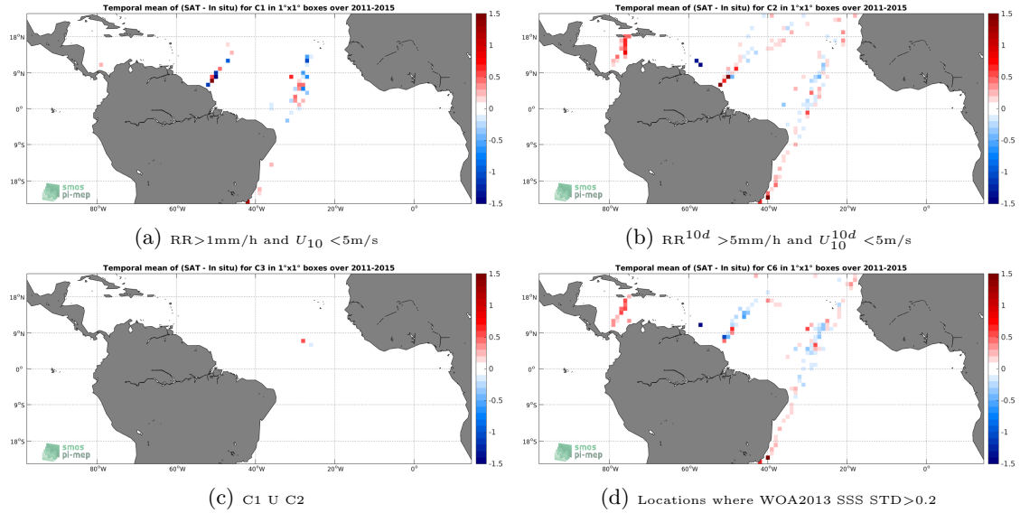
Figure 12: Temporal mean gridded over spatial boxes of size 1^\circ \times 1^\circ of \Delta SSS (Aquarius-L3-JPL-V5-MONTHLY - TSG-LEGOS-DM) for 4 different subdatasets corresponding to: RR > 1\text{mm/h} and U_{10} < 5\text{m/s} (a), RR^{10d} > 5\text{mm/h} and U_{10}^{10d} < 5\text{m/s} (b), C1 U C2 (c), Locations where WOA2013 SSS STD > 0.2 (d).
