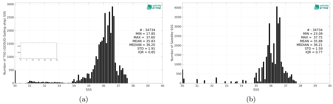
Figure 2: Histograms of SSS from TSG (GOSUD-Sailing-ship) (a) and Aquarius SSS L3 CAP v5 - Monthly (JPL) (b) considering all match-up pairs per bins of 0.1 over the Tropical Atlantic Ocean Pi-MEP region and for the full satellite product period.
