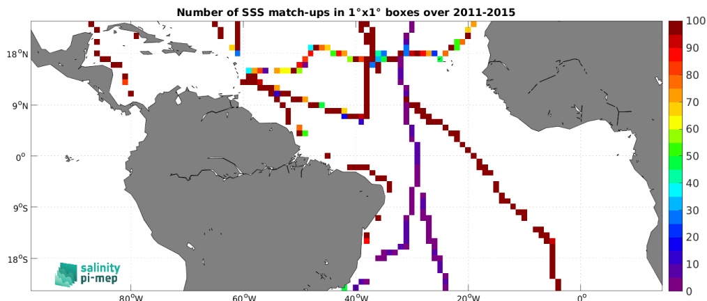
Figure 4: Number of SSS match-ups between TSG (GOSUD-Sailing-ship) SSS and the Aquarius SSS L3 CAP v5 - Monthly (JPL) SSS product for the Tropical Atlantic Ocean Pi-MEP region over 1^\circ \times 1^\circ boxes and for the full satellite product period.
