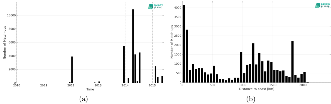
Figure 1: Number of match-ups between TSG (GOSUD-Sailing-ship) and Aquarius SSS L3 CAP v5 - Monthly (JPL) SSS as a function of time (a) and as function of the distance to coast (b) over the Tropical Atlantic Ocean Pi-MEP region and for the full satellite product period.
