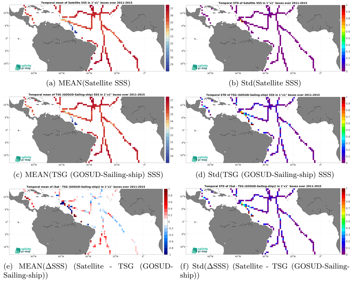
Figure 6: Temporal mean (left) and Std (right) of SSS from Aquarius SSS L3 CAP v5 - Monthly (JPL) (top), TSG (GOSUD-Sailing-ship) (middle), and of \Delta SSS (Satellite - TSG (GOSUD-Sailing-ship)). Only match-up pairs are used to generate these maps.
