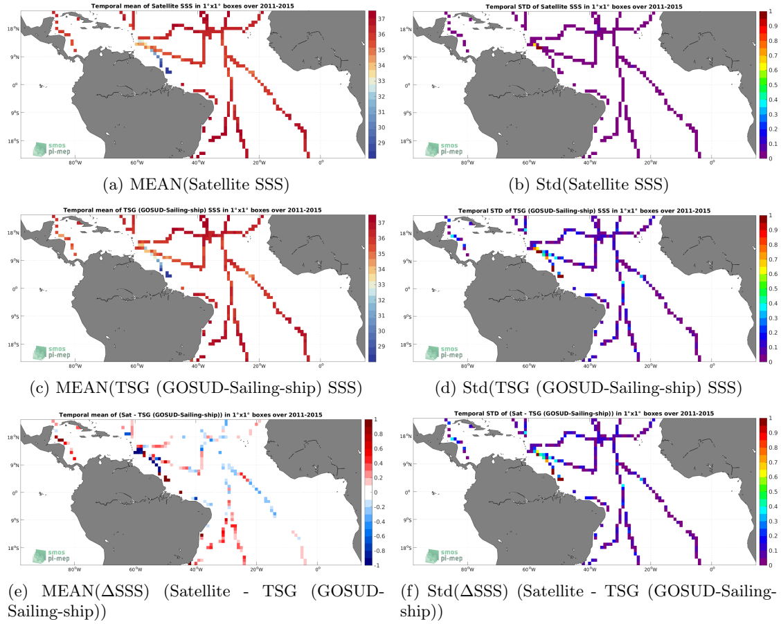
Figure 6: Temporal mean (left) and Std (right) of SSS from Aquarius SSS L3 CAP v5 - Monthly (JPL) (top), TSG (GOSUD-Sailing-ship) (middle), and of \Delta SSS (Satellite - TSG (GOSUD-Sailing-ship)). Only match-up pairs are used to generate these maps.
