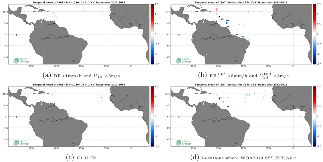
Figure 12: Temporal mean gridded over spatial boxes of size 1^\circ \times 1^\circ of \Delta SSS (Aquarius-L3-JPL-V5-MONTHLY - TSG-GOSUD-Sailing-ship) for 4 different subdatasets corresponding to: RR > 1\text{mm/h} and U_{10} < 5\text{m/s} (a), RR^{10d} > 5\text{mm/h} and U_{10}^{10d} < 5\text{m/s} (b), C1 U C2 (c), Locations where WOA2013 SSS STD > 0.2 (d).
