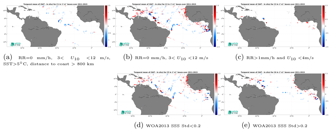
Figure 14: Temporal mean gridded over spatial boxes of size 1^\circ \times 1^\circ of \Delta SSS (Aquarius SSS L3 CAP v5 - Monthly (JPL) - TSG (GOSUD-Research-vessel)) for 5 different subdatasets corresponding to:RR=0 mm/h, 3 < U_{10} < 12 m/s, SST >5^\circ\text{C} , distance to coast > 800 km (a), RR=0 mm/h, 3 < U_{10} < 12 m/s (b), RR >1 mm/h and U_{10} < 4 m/s (c), WOA2013 SSS Std <0.2 (d), WOA2013 SSS Std >0.2 (e).
