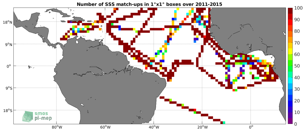
Figure 4: Number of SSS match-ups between TSG (GOSUD-Research-vessel) SSS and the Aquarius SSS L3 CAP v5 - Monthly (JPL) SSS product for the Tropical Atlantic Ocean Pi-MEP region over 1°x1° boxes and for the full satellite product period.
