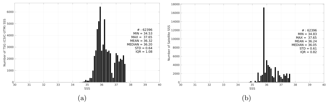
Figure 3: Histograms of SSS from TSG (CSIC-UTM) (a) and Aquarius SSS L3 CAP v5 - Monthly (JPL) (b) considering all match-up pairs per bins of 0.1 over the Tropical Atlantic Ocean Pi-MEP region and for the full satellite product period.
