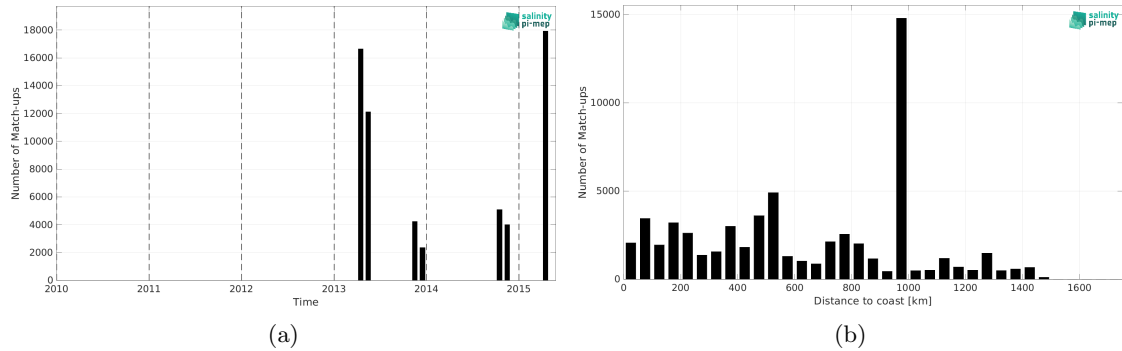
Figure 2: Number of match-ups between TSG (CSIC-UTM) and Aquarius SSS L3 CAP v5 - Monthly (JPL) SSS as a function of time (a) and as function of the distance to coast (b) over the Tropical Atlantic Ocean Pi-MEP region and for the full satellite product period.
