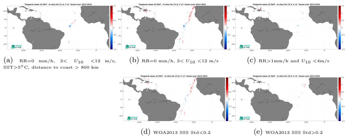
Figure 14: Temporal mean gridded over spatial boxes of size 1^\circ \times 1^\circ of \Delta SSS (Aquarius SSS L3 CAP v5 - Monthly (JPL) - TSG (CSIC-UTM)) for 5 different subdatasets corresponding to:RR=0 mm/h, 3 < U_{10} < 12 m/s, SST >5^\circ\text{C} , distance to coast > 800 km (a), RR=0 mm/h, 3 < U_{10} < 12 m/s (b), RR >1 mm/h and U_{10} < 4 m/s (c), WOA2013 SSS Std <0.2 (d), WOA2013 SSS Std >0.2 (e).
