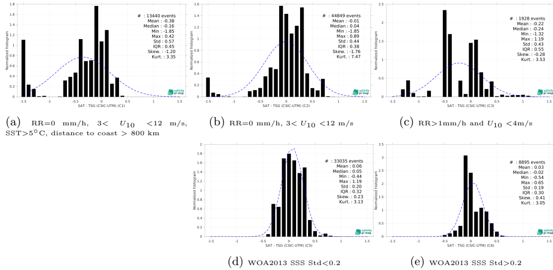
Figure 15: Normalized histogram of \Delta SSS (Aquarius SSS L3 CAP v5 - Monthly (JPL) - TSG (CSIC-UTM)) for 5 different subdatasets corresponding to: RR=0 mm/h, 3 < U_{10} < 12 m/s, SST > 5°C, distance to coast > 800 km (a), RR=0 mm/h, 3 < U_{10} < 12 m/s (b), RR > 1mm/h and U_{10} < 4 m/s (c), WOA2013 SSS Std < 0.2 (d), WOA2013 SSS Std > 0.2 (e).
