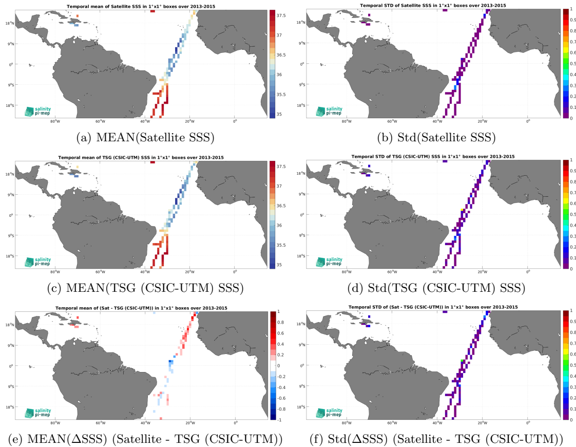
Figure 7: Temporal mean (left) and Std (right) of SSS from Aquarius SSS L3 CAP v5 - Monthly (JPL) (top), TSG (CSIC-UTM) (middle), and of \Delta SSS (Satellite - TSG (CSIC-UTM)). Only match-up pairs are used to generate these maps.
