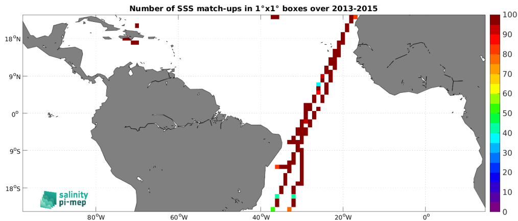
Figure 5: Number of SSS match-ups between TSG (CSIC-UTM) SSS and the Aquarius SSS L3 CAP v5 - Monthly (JPL) SSS product for the Tropical Atlantic Ocean Pi-MEP region over 1^\circ \times 1^\circ boxes and for the full satellite product period.
